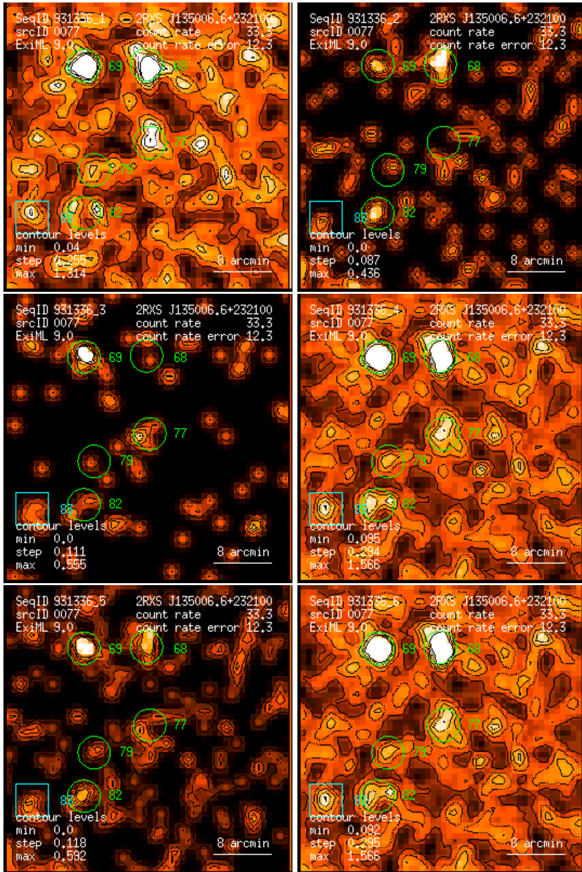
Figure 77: RASS 931336: detection 0077: band rate images, Gaussian filter: (1) PSPC channels 11 – 41, (2) 52 – 90, (3) 91 – 201, (4) 11 – 235, (5) 52 – 201, (6) 11 – 201. Broad band rates in counts/ks. Band rate contour levels in counts/ks/arcmin 2 .
