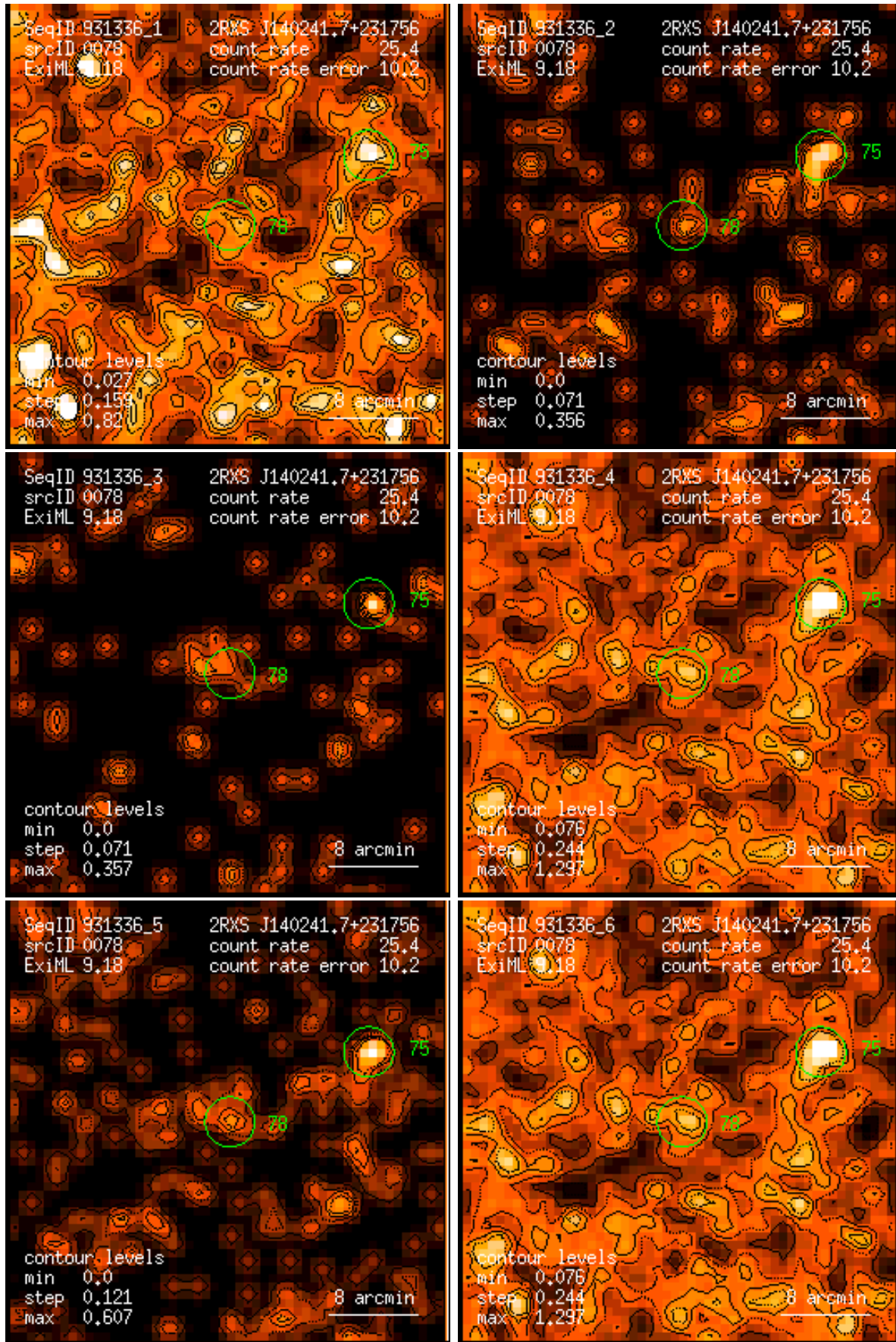
Figure 78: RASS 931336: detection 0078: band rate images, Gaussian filter: (1) PSPC channels 11 – 41, (2) 52 – 90, (3) 91 – 201, (4) 11 – 235, (5) 52 – 201, (6) 11 – 201. Broad band rates in counts/ks. Band rate contour levels in counts/ks/arcmin 2 .
