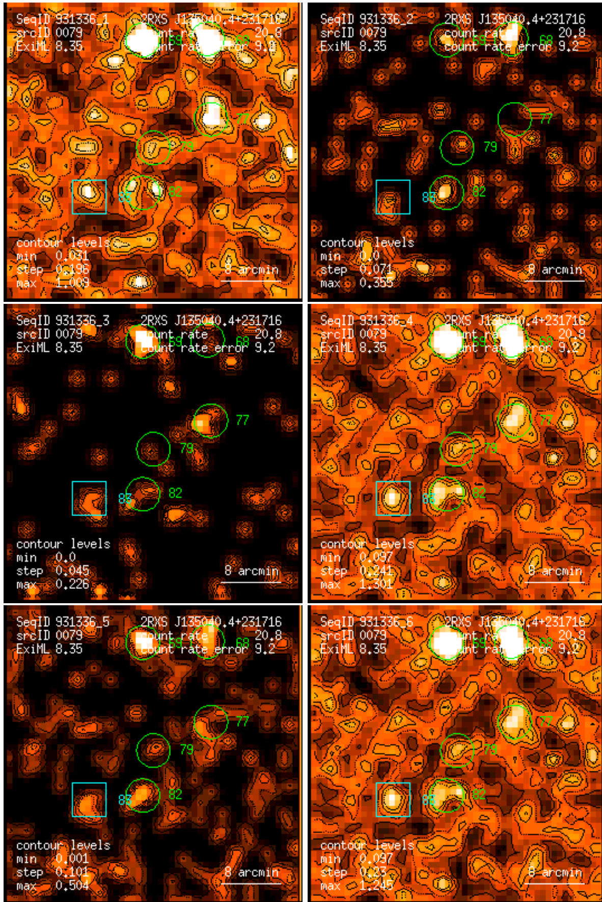
Figure 79: RASS 931336: detection 0079: band rate images, Gaussian filter: (1) PSPC channels 11 – 41, (2) 52 – 90, (3) 91 – 201, (4) 11 – 235, (5) 52 – 201, (6) 11 – 201. Broad band rates in counts/ks. Band rate contour levels in counts/ks/arcmin 2 .
