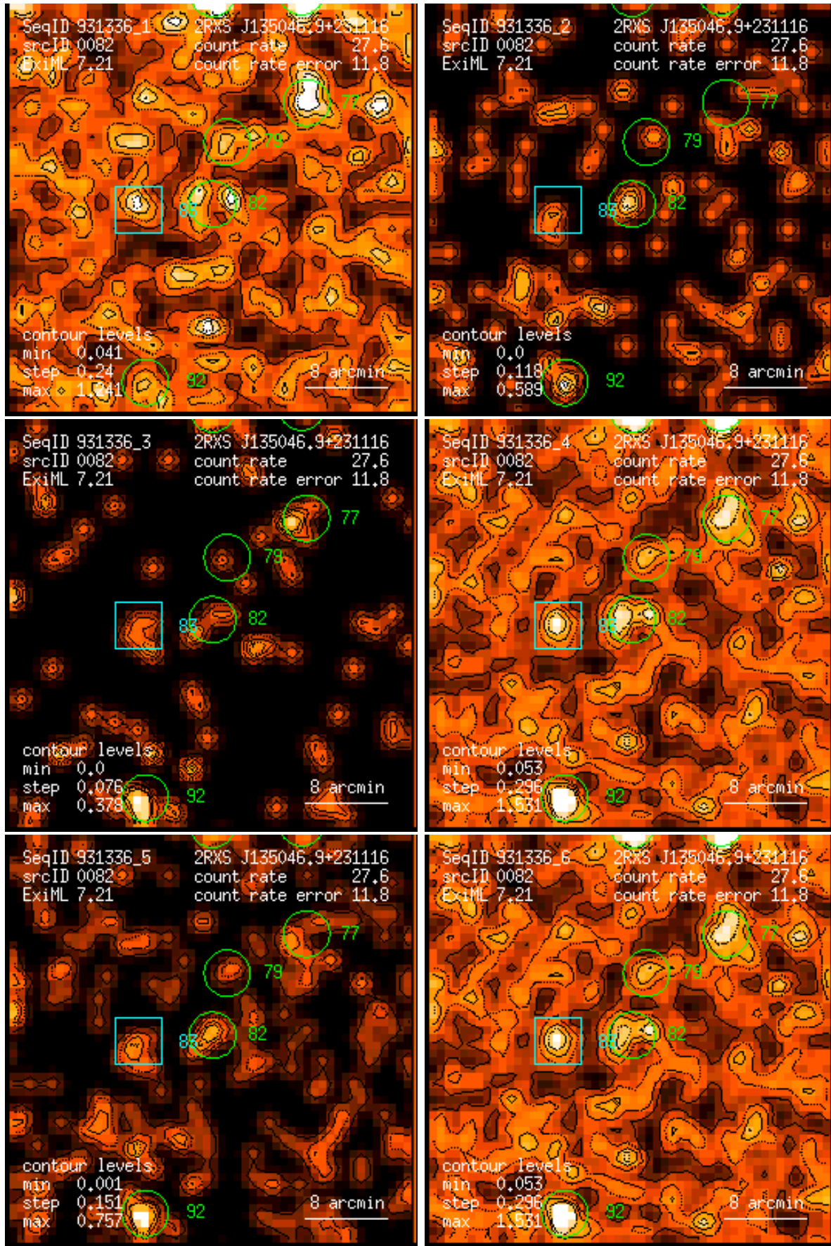
Figure 82: RASS 931336: detection 0082: band rate images, Gaussian filter: (1) PSPC channels 11 – 41, (2) 52 – 90, (3) 91 – 201, (4) 11 – 235, (5) 52 – 201, (6) 11 – 201. Broad band rates in counts/ks. Band rate contour levels in counts/ks/arcmin 2 .
