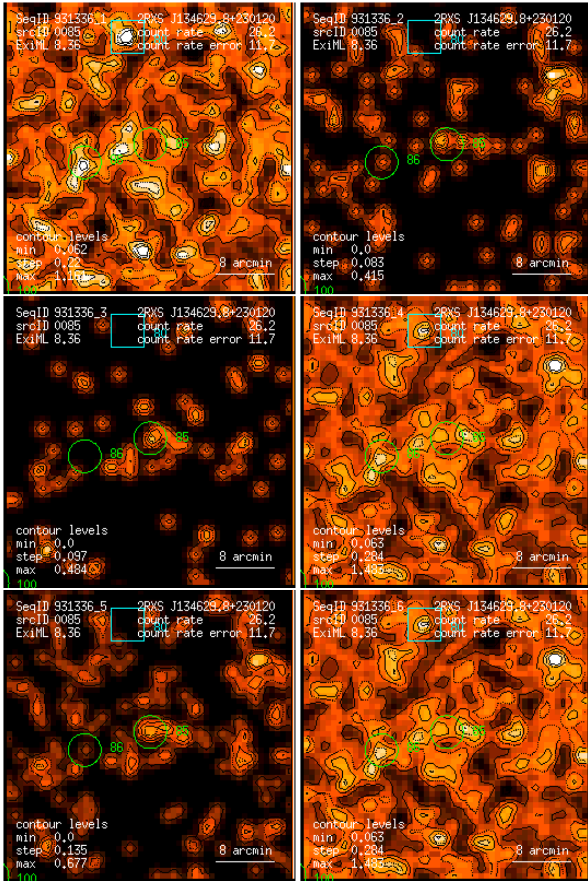
Figure 85: RASS 931336: detection 0085: band rate images, Gaussian filter: (1) PSPC channels 11 – 41, (2) 52 – 90, (3) 91 – 201, (4) 11 – 235, (5) 52 – 201, (6) 11 – 201. Broad band rates in counts/ks. Band rate contour levels in counts/ks/arcmin 2 .
