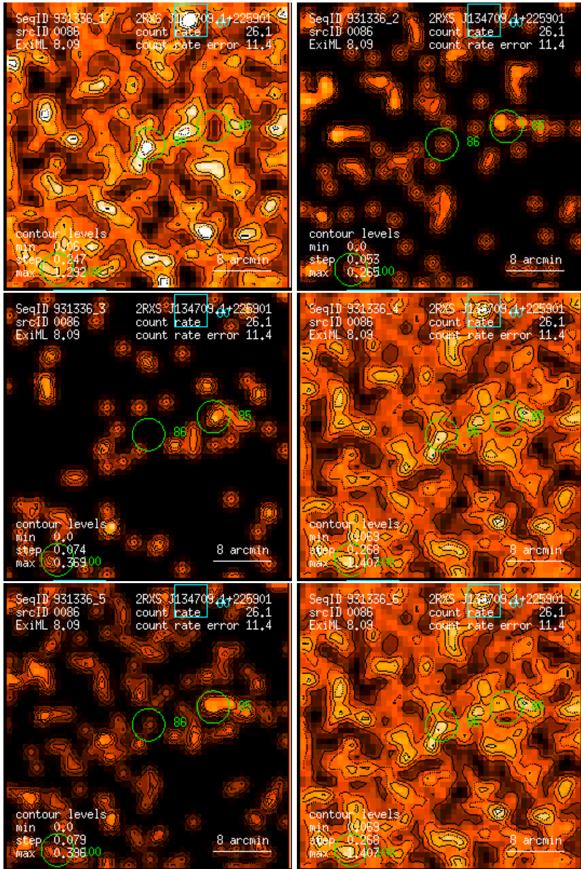
Figure 86: RASS 931336: detection 0086: band rate images, Gaussian filter: (1) PSPC channels 11 – 41, (2) 52 – 90, (3) 91 – 201, (4) 11 – 235, (5) 52 – 201, (6) 11 – 201. Broad band rates in counts/ks. Band rate contour levels in counts/ks/arcmin 2 .
