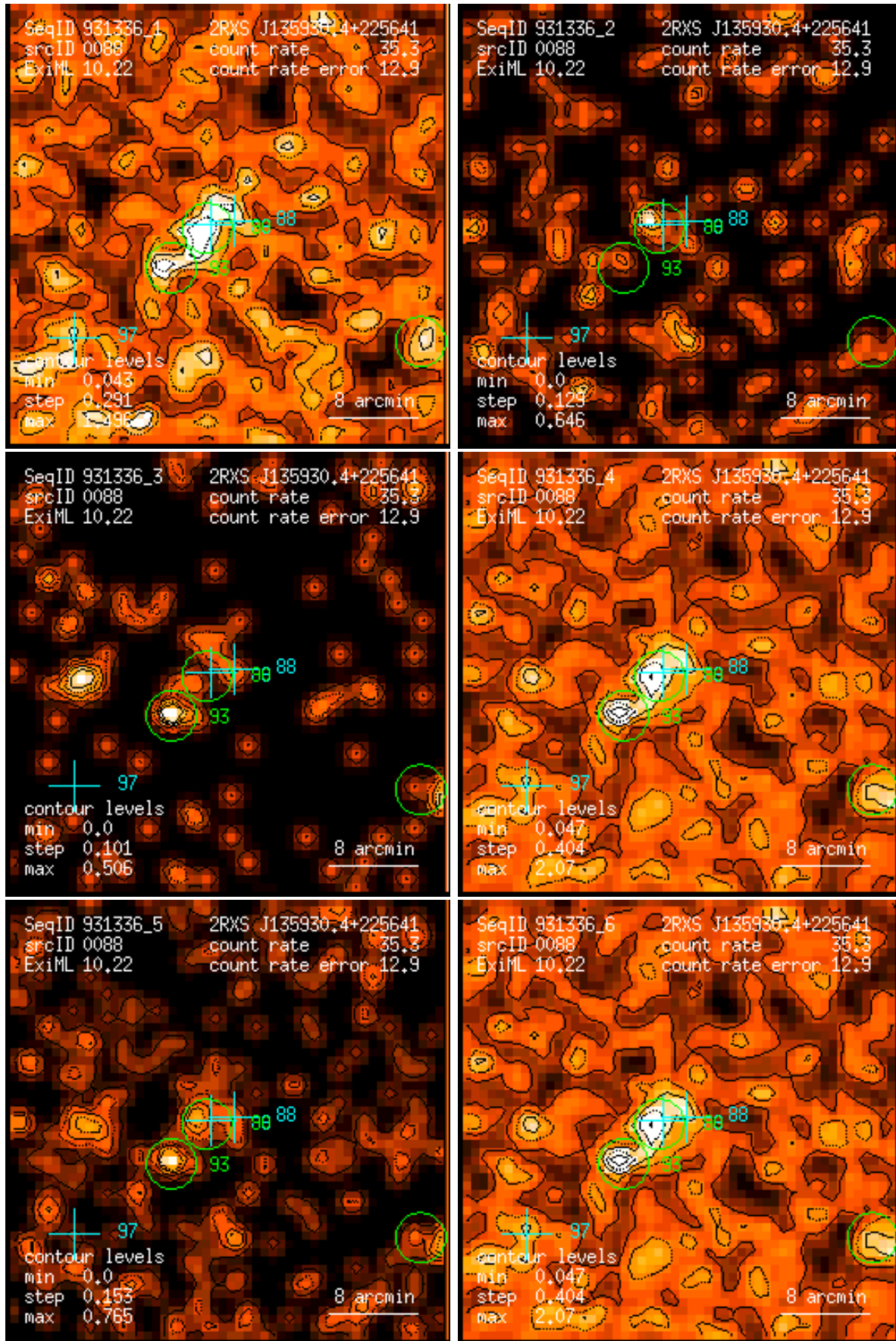
Figure 88: RASS 931336: detection 0088: band rate images, Gaussian filter: (1) PSPC channels 11 – 41, (2) 52 – 90, (3) 91 – 201, (4) 11 – 235, (5) 52 – 201, (6) 11 – 201. Broad band rates in counts/ks. Band rate contour levels in counts/ks/arcmin 2 .
