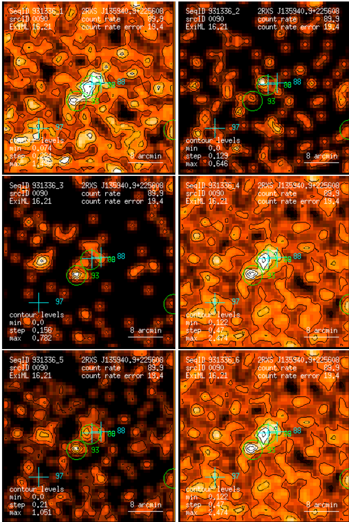
Figure 90: RASS 931336: detection 0090: band rate images, Gaussian filter: (1) PSPC channels 11 – 41, (2) 52 – 90, (3) 91 – 201, (4) 11 – 235, (5) 52 – 201, (6) 11 – 201. Broad band rates in counts/ks. Band rate contour levels in counts/ks/arcmin 2 .
