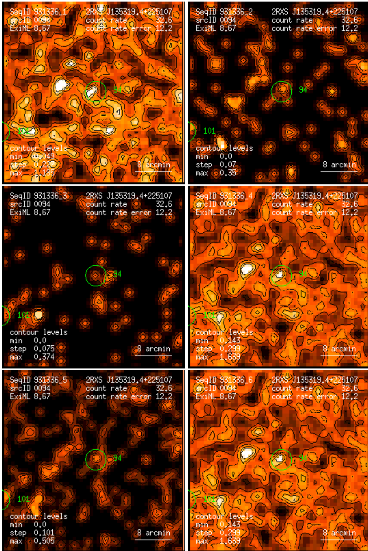
Figure 94: RASS 931336: detection 0094: band rate images, Gaussian filter: (1) PSPC channels 11 – 41, (2) 52 – 90, (3) 91 – 201, (4) 11 – 235, (5) 52 – 201, (6) 11 – 201. Broad band rates in counts/ks. Band rate contour levels in counts/ks/arcmin 2 .
