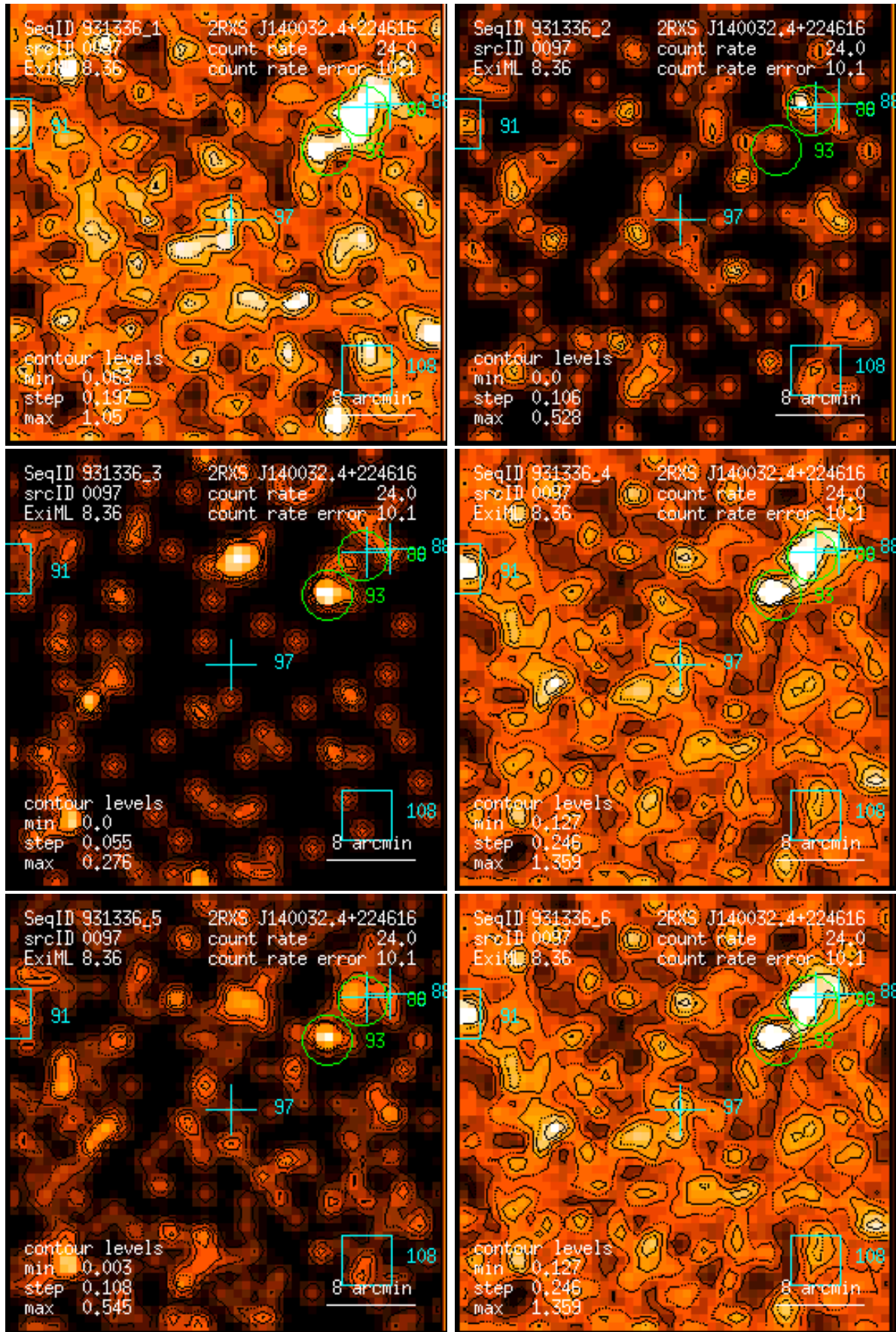
Figure 97: RASS 931336: detection 0097: band rate images, Gaussian filter: (1) PSPC channels 11 – 41, (2) 52 – 90, (3) 91 – 201, (4) 11 – 235, (5) 52 – 201, (6) 11 – 201. Broad band rates in counts/ks. Band rate contour levels in counts/ks/arcmin 2 .
