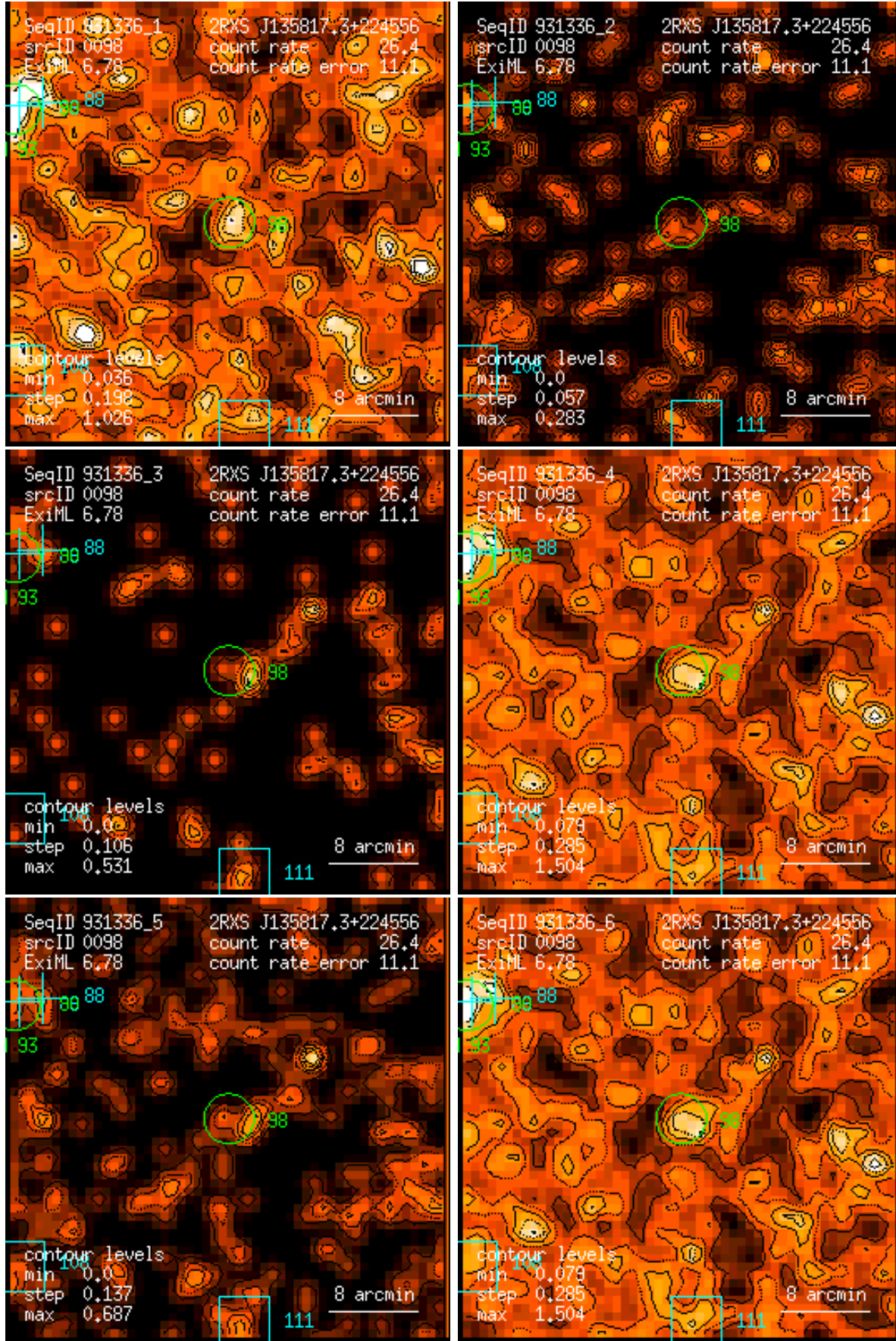
Figure 98: RASS 931336: detection 0098: band rate images, Gaussian filter: (1) PSPC channels 11 – 41, (2) 52 – 90, (3) 91 – 201, (4) 11 – 235, (5) 52 – 201, (6) 11 – 201. Broad band rates in counts/ks. Band rate contour levels in counts/ks/arcmin 2 .
