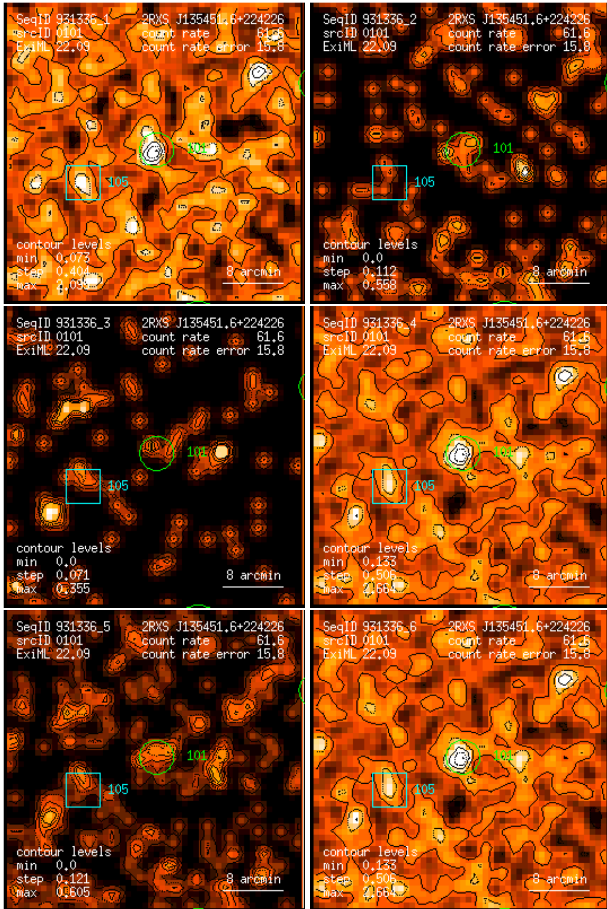
Figure 101: RASS 931336: detection 0101: band rate images, Gaussian filter: (1) PSPC channels 11 – 41, (2) 52 – 90, (3) 91 – 201, (4) 11 – 235, (5) 52 – 201, (6) 11 – 201. Broad band rates in counts/ks. Band rate contour levels in counts/ks/arcmin 2 .
