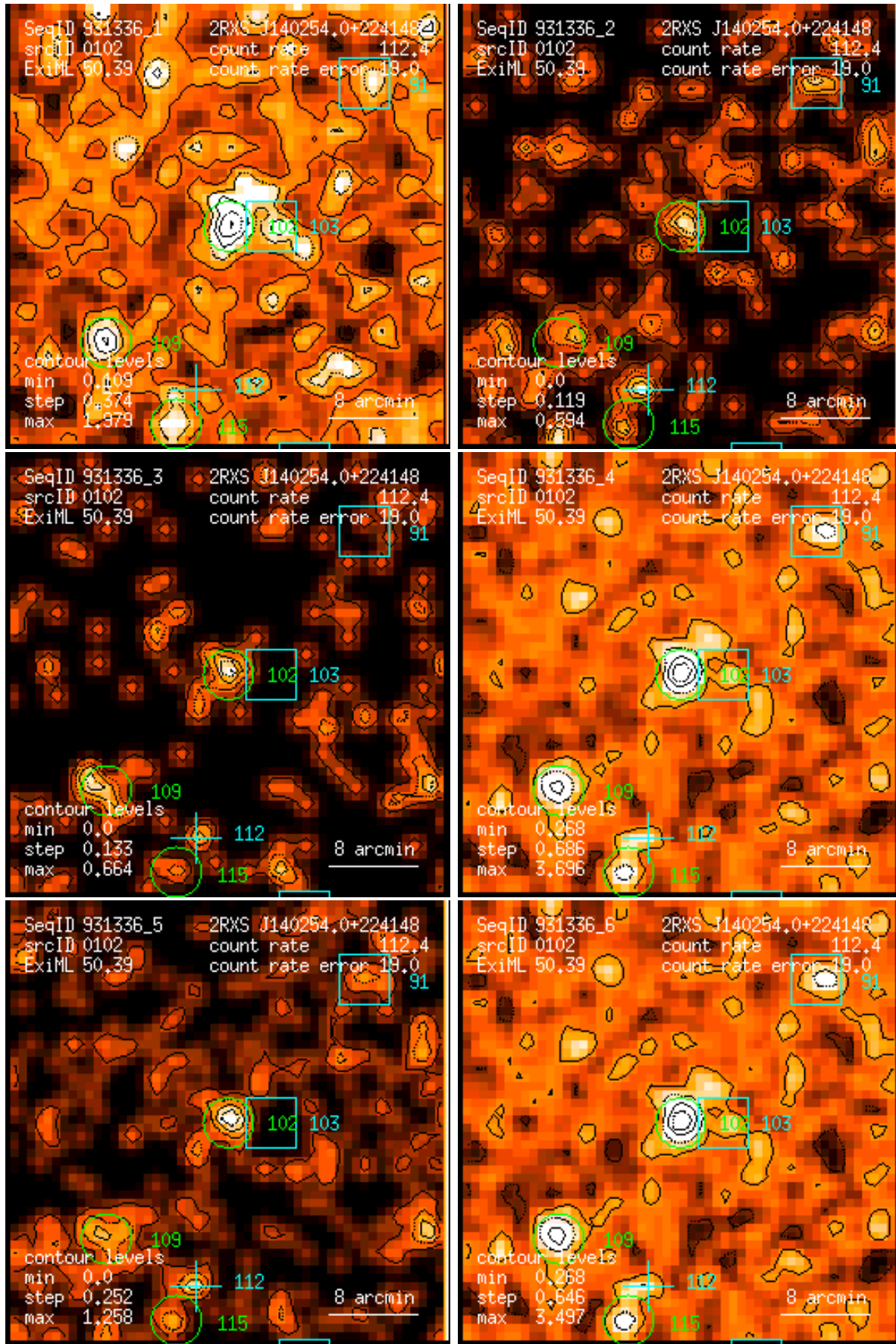
Figure 102: RASS 931336: detection 0102: band rate images, Gaussian filter: (1) PSPC channels 11 – 41, (2) 52 – 90, (3) 91 – 201, (4) 11 – 235, (5) 52 – 201, (6) 11 – 201. Broad band rates in counts/ks. Band rate contour levels in counts/ks/arcmin 2 .
