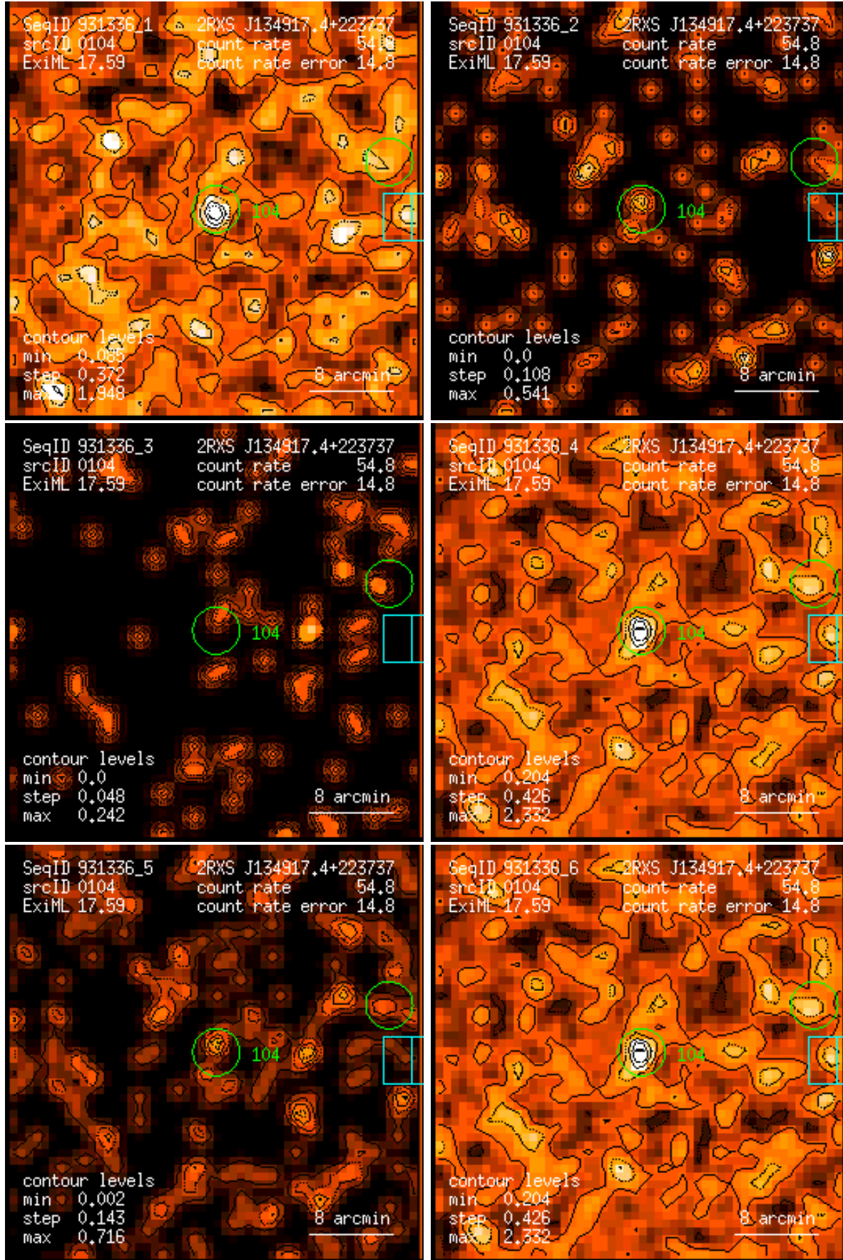
Figure 104: RASS 931336: detection 0104: band rate images, Gaussian filter: (1) PSPC channels 11 – 41, (2) 52 – 90, (3) 91 – 201, (4) 11 – 235, (5) 52 – 201, (6) 11 – 201. Broad band rates in counts/ks. Band rate contour levels in counts/ks/arcmin 2 .
