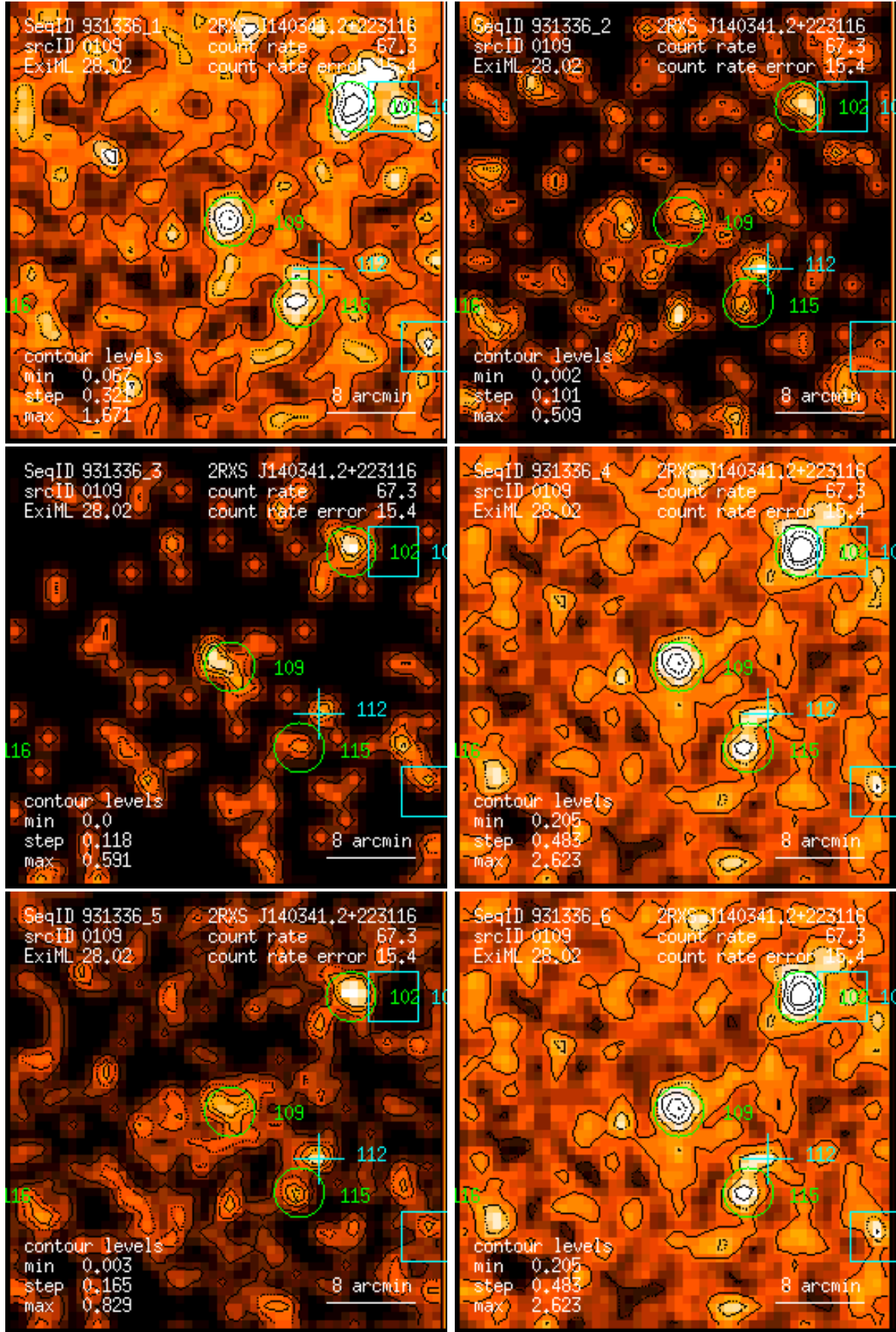
Figure 109: RASS 931336: detection 0109: band rate images, Gaussian filter: (1) PSPC channels 11 – 41, (2) 52 – 90, (3) 91 – 201, (4) 11 – 235, (5) 52 – 201, (6) 11 – 201. Broad band rates in counts/ks. Band rate contour levels in counts/ks/arcmin 2 .
