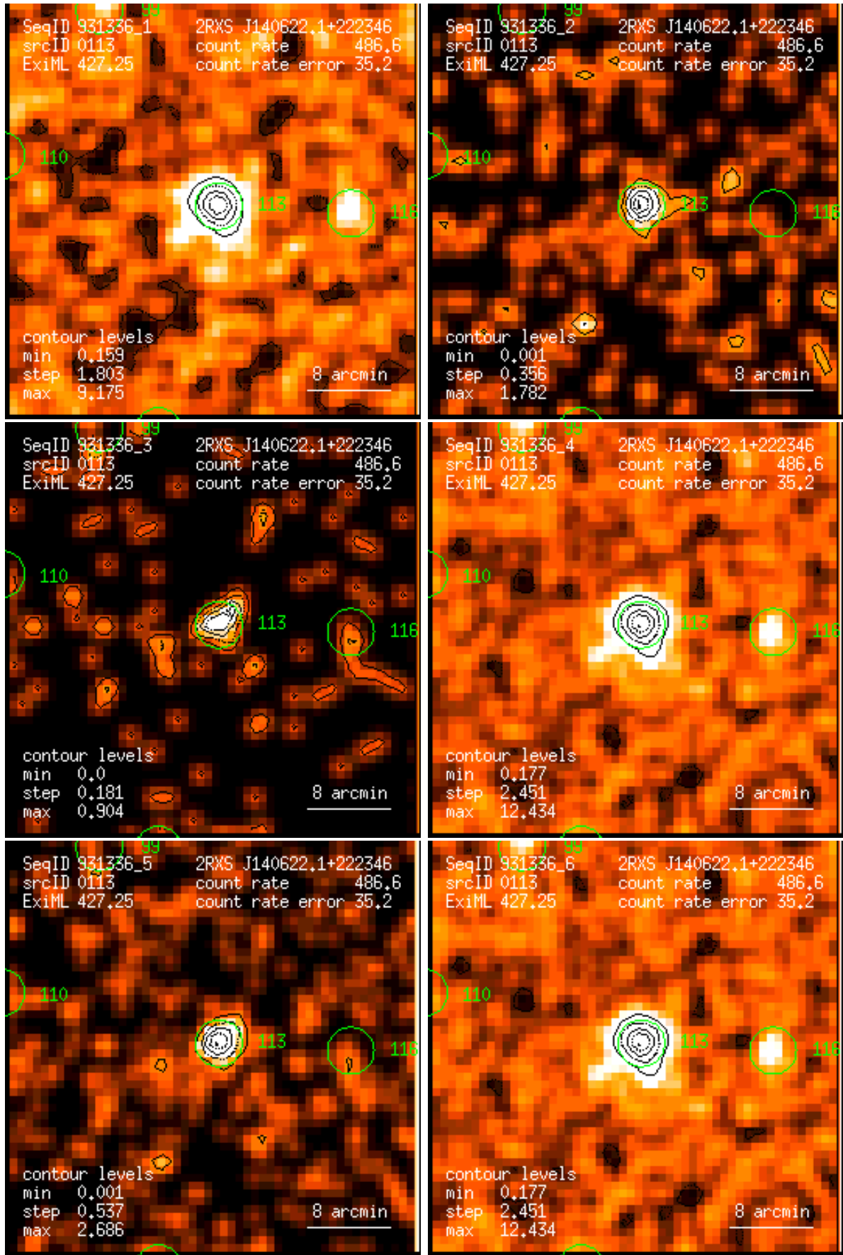
Figure 113: RASS 931336: detection 0113: band rate images, Gaussian filter: (1) PSPC channels 11 – 41, (2) 52 – 90, (3) 91 – 201, (4) 11 – 235, (5) 52 – 201, (6) 11 – 201. Broad band rates in counts/ks. Band rate contour levels in counts/ks/arcmin 2 .
