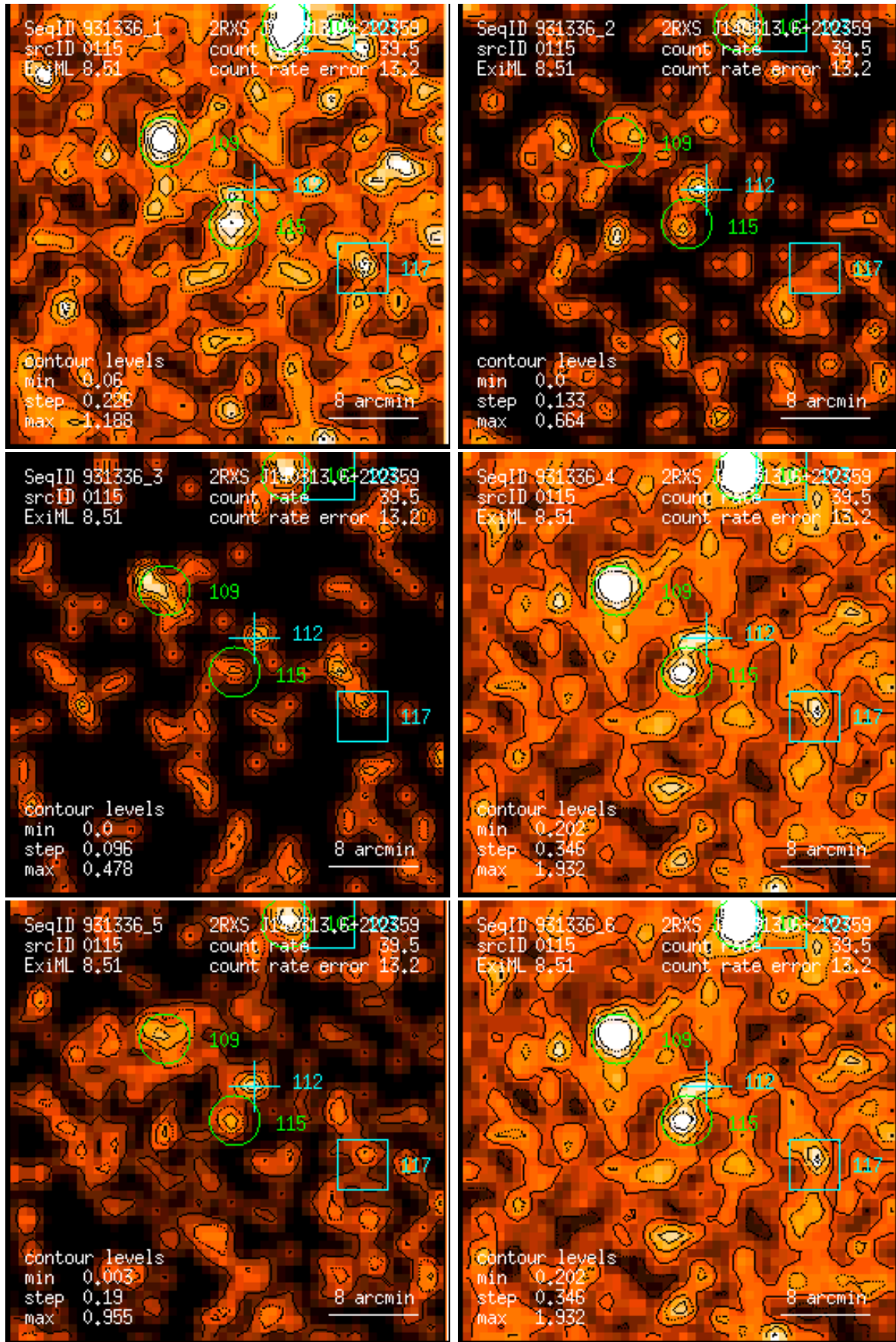
Figure 115: RASS 931336: detection 0115: band rate images, Gaussian filter: (1) PSPC channels 11 – 41, (2) 52 – 90, (3) 91 – 201, (4) 11 – 235, (5) 52 – 201, (6) 11 – 201. Broad band rates in counts/ks. Band rate contour levels in counts/ks/arcmin 2 .
