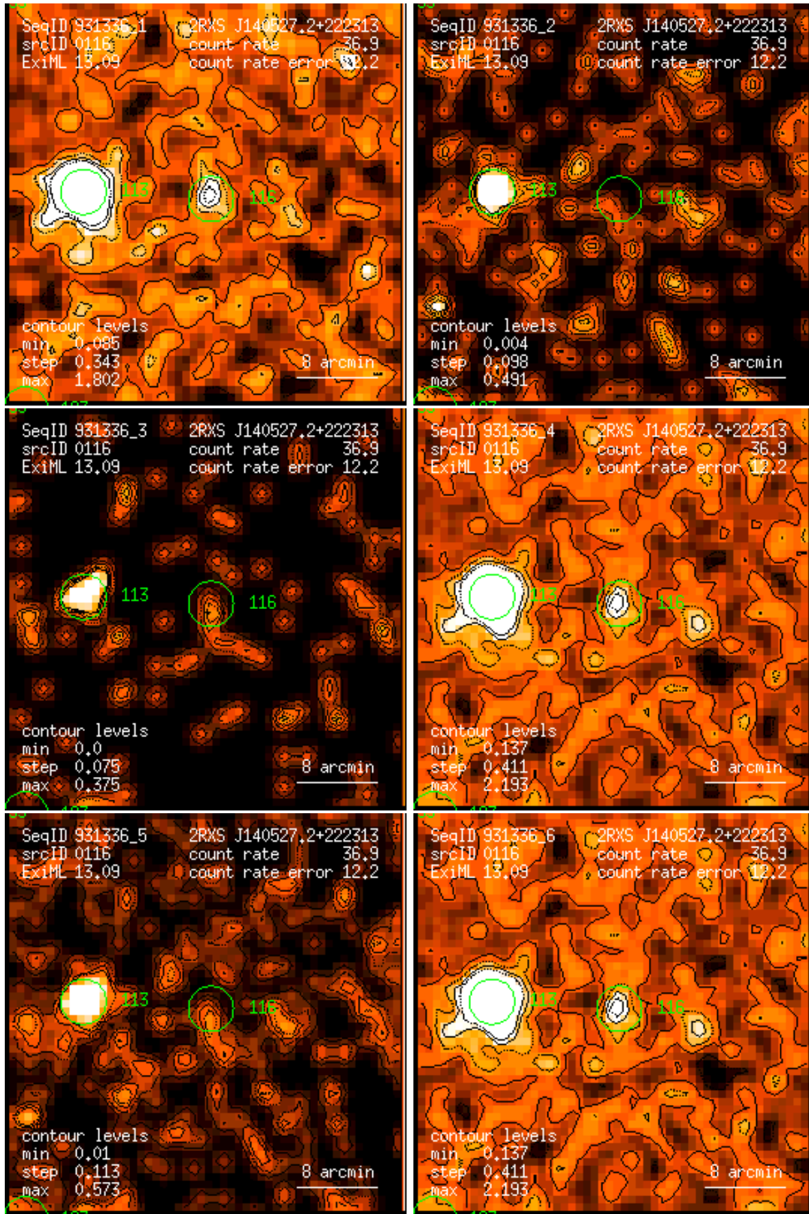
Figure 116: RASS 931336: detection 0116: band rate images, Gaussian filter: (1) PSPC channels 11 – 41, (2) 52 – 90, (3) 91 – 201, (4) 11 – 235, (5) 52 – 201, (6) 11 – 201. Broad band rates in counts/ks. Band rate contour levels in counts/ks/arcmin 2 .
