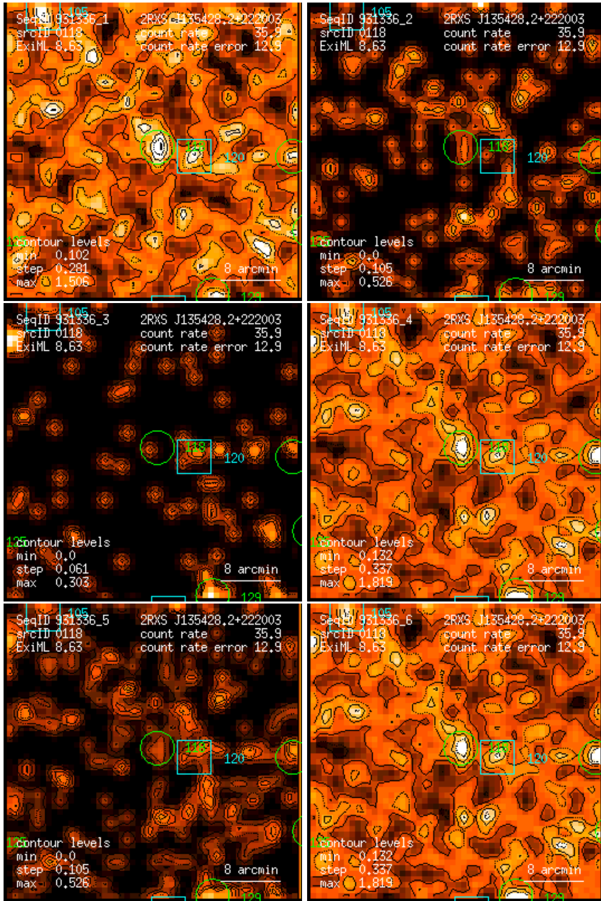
Figure 118: RASS 931336: detection 0118: band rate images, Gaussian filter: (1) PSPC channels 11 – 41, (2) 52 – 90, (3) 91 – 201, (4) 11 – 235, (5) 52 – 201, (6) 11 – 201. Broad band rates in counts/ks. Band rate contour levels in counts/ks/arcmin 2 .
