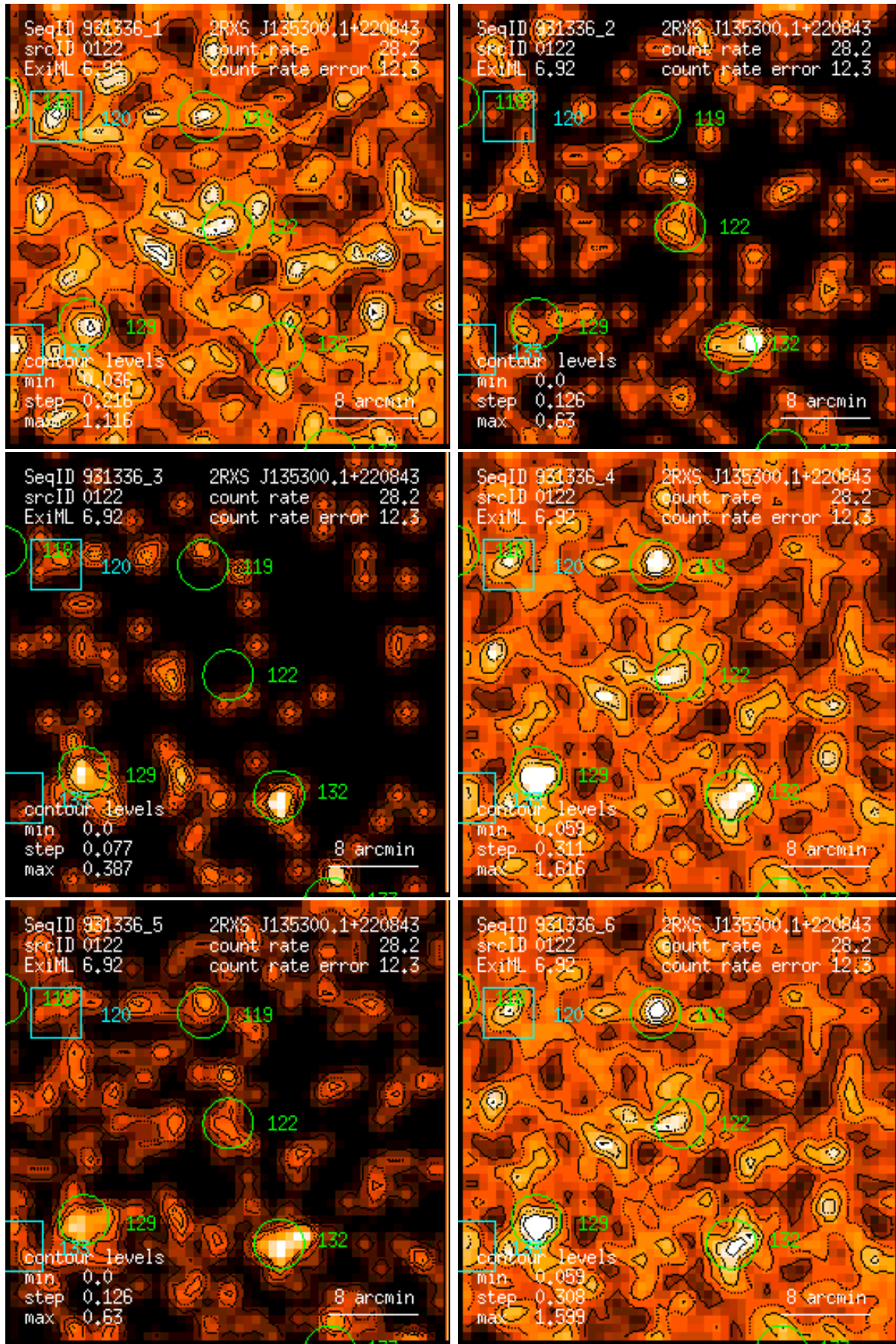
Figure 122: RASS 931336: detection 0122: band rate images, Gaussian filter: (1) PSPC channels 11 – 41, (2) 52 – 90, (3) 91 – 201, (4) 11 – 235, (5) 52 – 201, (6) 11 – 201. Broad band rates in counts/ks. Band rate contour levels in counts/ks/arcmin 2 .
