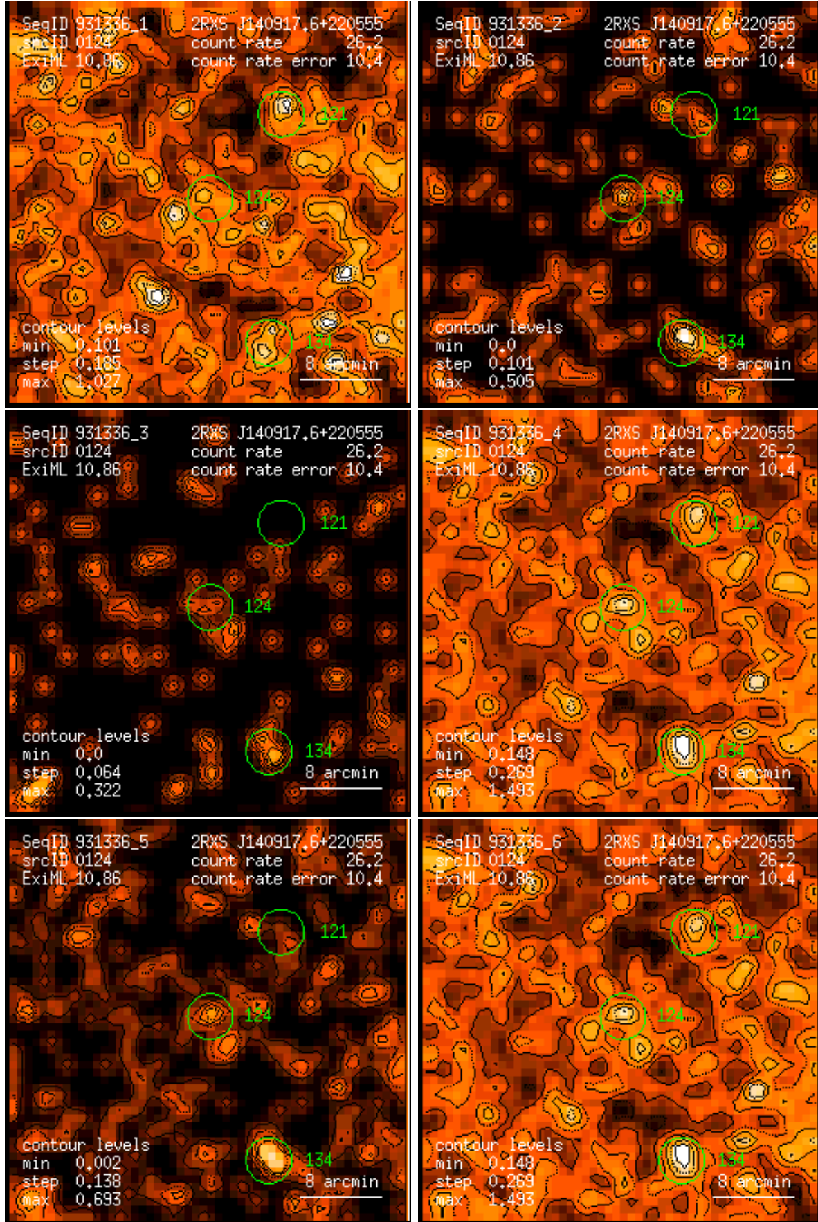
Figure 124: RASS 931336: detection 0124: band rate images, Gaussian filter: (1) PSPC channels 11 – 41, (2) 52 – 90, (3) 91 – 201, (4) 11 – 235, (5) 52 – 201, (6) 11 – 201. Broad band rates in counts/ks. Band rate contour levels in counts/ks/arcmin 2 .
