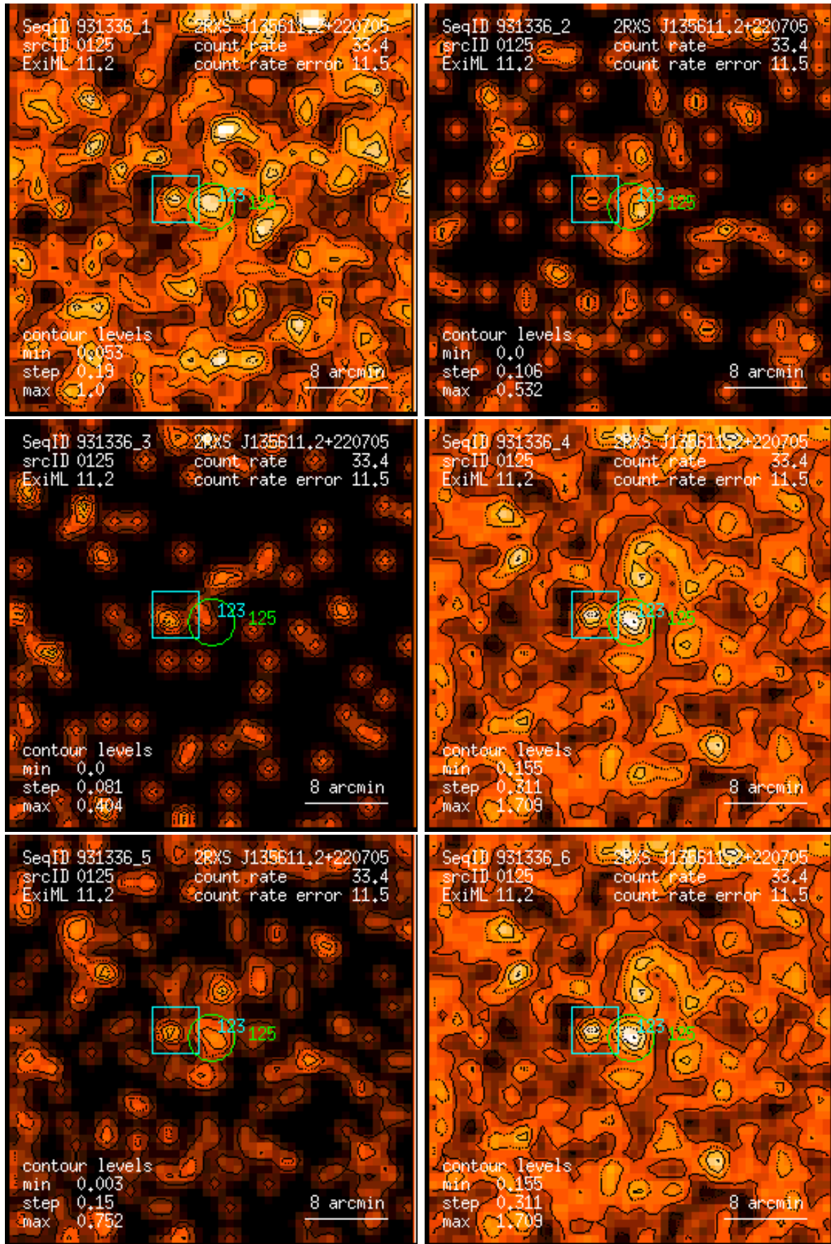
Figure 125: RASS 931336: detection 0125: band rate images, Gaussian filter: (1) PSPC channels 11 – 41, (2) 52 – 90, (3) 91 – 201, (4) 11 – 235, (5) 52 – 201, (6) 11 – 201. Broad band rates in counts/ks. Band rate contour levels in counts/ks/arcmin 2 .
