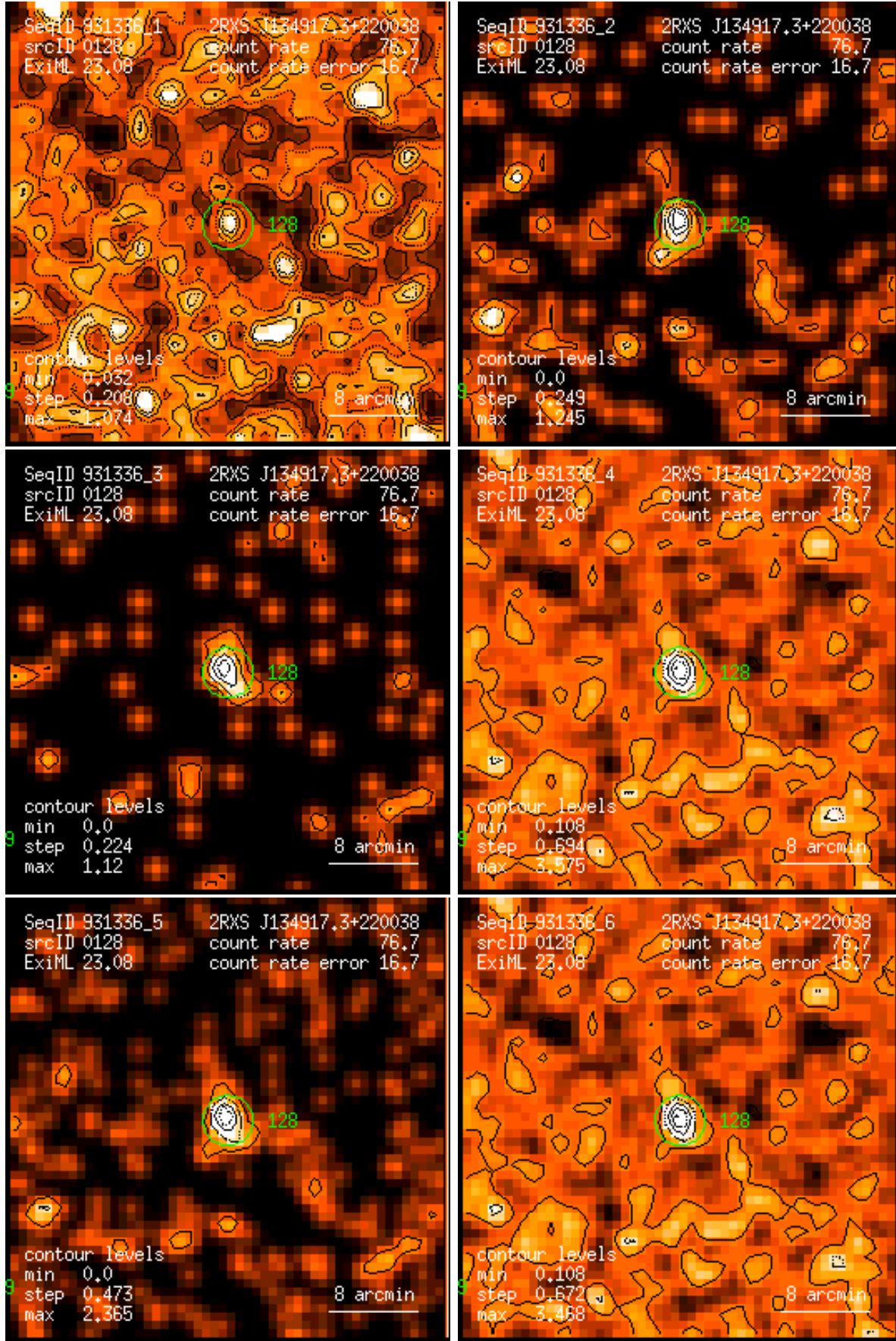
Figure 128: RASS 931336: detection 0128: band rate images, Gaussian filter: (1) PSPC channels 11 – 41, (2) 52 – 90, (3) 91 – 201, (4) 11 – 235, (5) 52 – 201, (6) 11 – 201. Broad band rates in counts/ks. Band rate contour levels in counts/ks/arcmin 2 .
