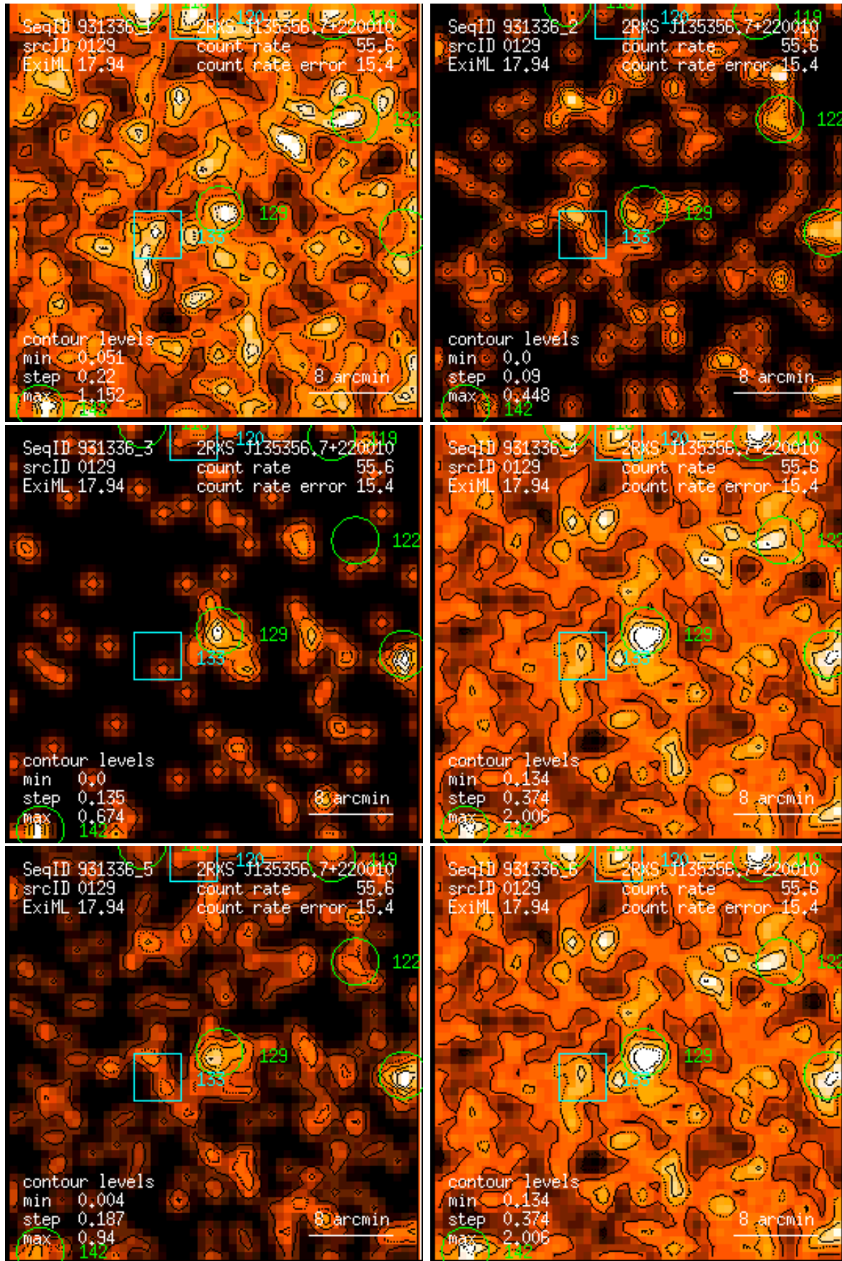
Figure 129: RASS 931336: detection 0129: band rate images, Gaussian filter: (1) PSPC channels 11 – 41, (2) 52 – 90, (3) 91 – 201, (4) 11 – 235, (5) 52 – 201, (6) 11 – 201. Broad band rates in counts/ks. Band rate contour levels in counts/ks/arcmin 2 .
