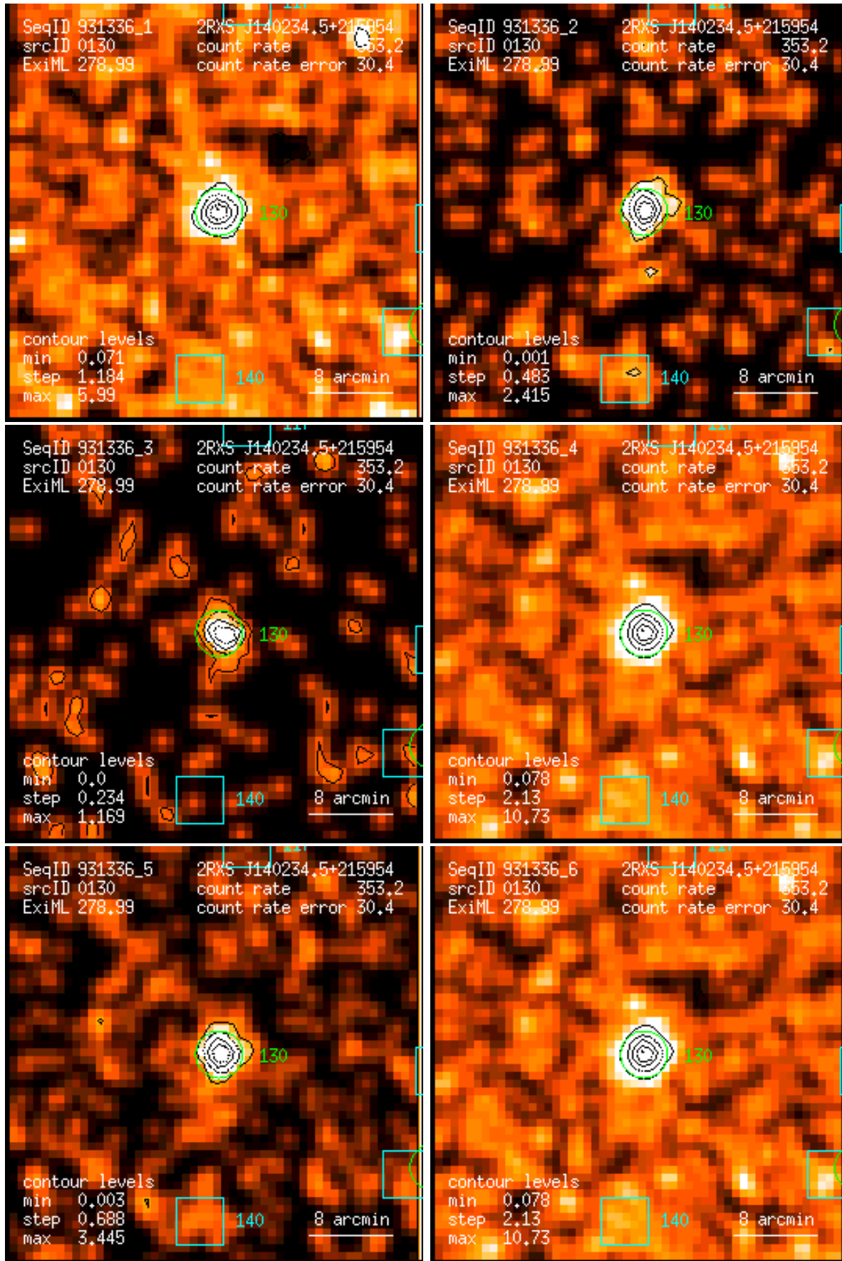
Figure 130: RASS 931336: detection 0130: band rate images, Gaussian filter: (1) PSPC channels 11 – 41, (2) 52 – 90, (3) 91 – 201, (4) 11 – 235, (5) 52 – 201, (6) 11 – 201. Broad band rates in counts/ks. Band rate contour levels in counts/ks/arcmin 2 .
