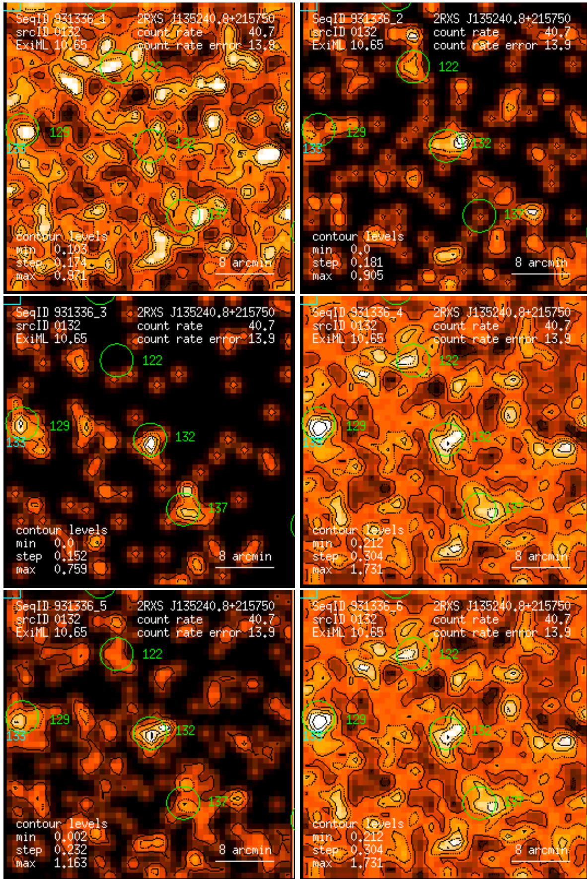
Figure 132: RASS 931336: detection 0132: band rate images, Gaussian filter: (1) PSPC channels 11 – 41, (2) 52 – 90, (3) 91 – 201, (4) 11 – 235, (5) 52 – 201, (6) 11 – 201. Broad band rates in counts/ks. Band rate contour levels in counts/ks/arcmin 2 .
