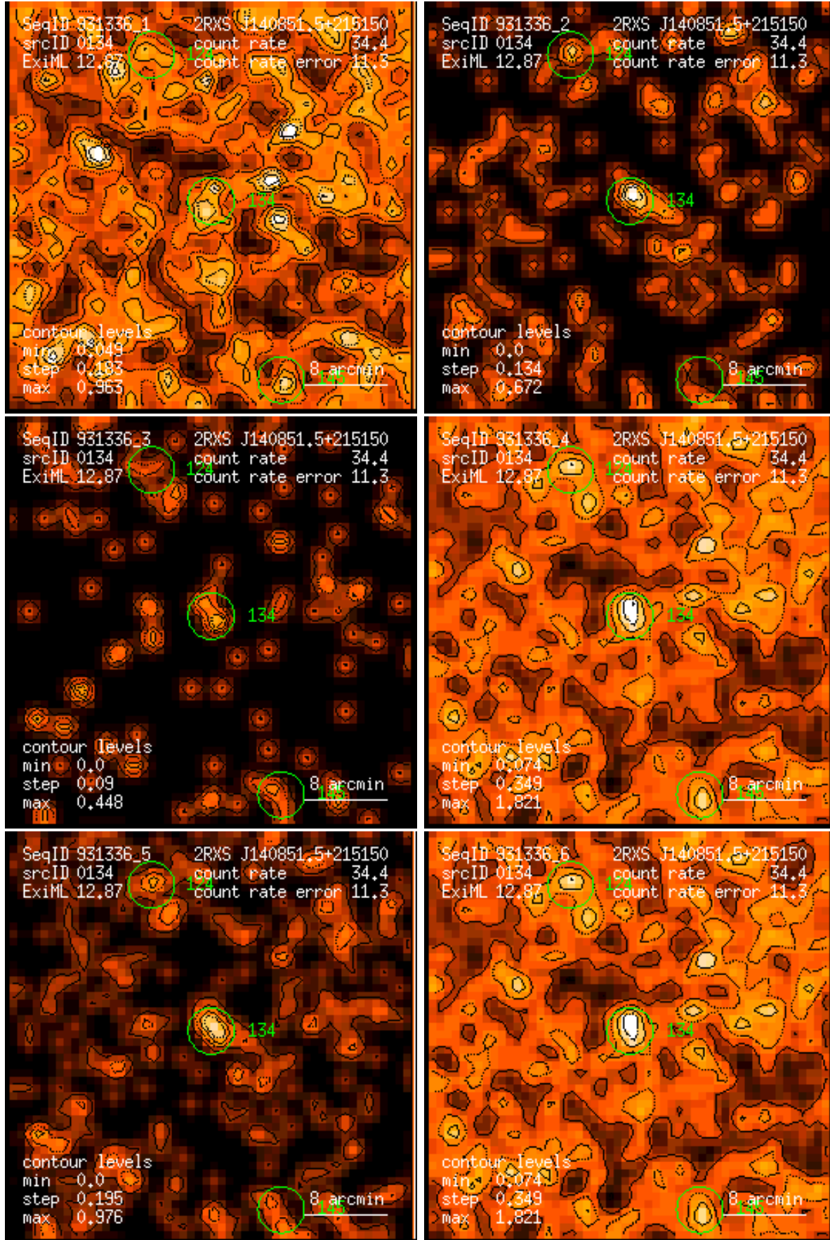
Figure 134: RASS 931336: detection 0134: band rate images, Gaussian filter: (1) PSPC channels 11 – 41, (2) 52 – 90, (3) 91 – 201, (4) 11 – 235, (5) 52 – 201, (6) 11 – 201. Broad band rates in counts/ks. Band rate contour levels in counts/ks/arcmin 2 .
