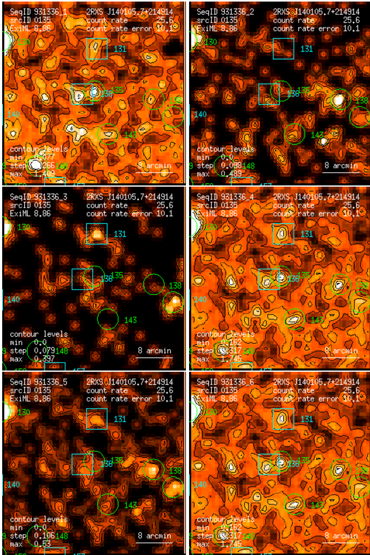
Figure 135: RASS 931336: detection 0135: band rate images, Gaussian filter: (1) PSPC channels 11 – 41, (2) 52 – 90, (3) 91 – 201, (4) 11 – 235, (5) 52 – 201, (6) 11 – 201. Broad band rates in counts/ks. Band rate contour levels in counts/ks/arcmin 2 .
