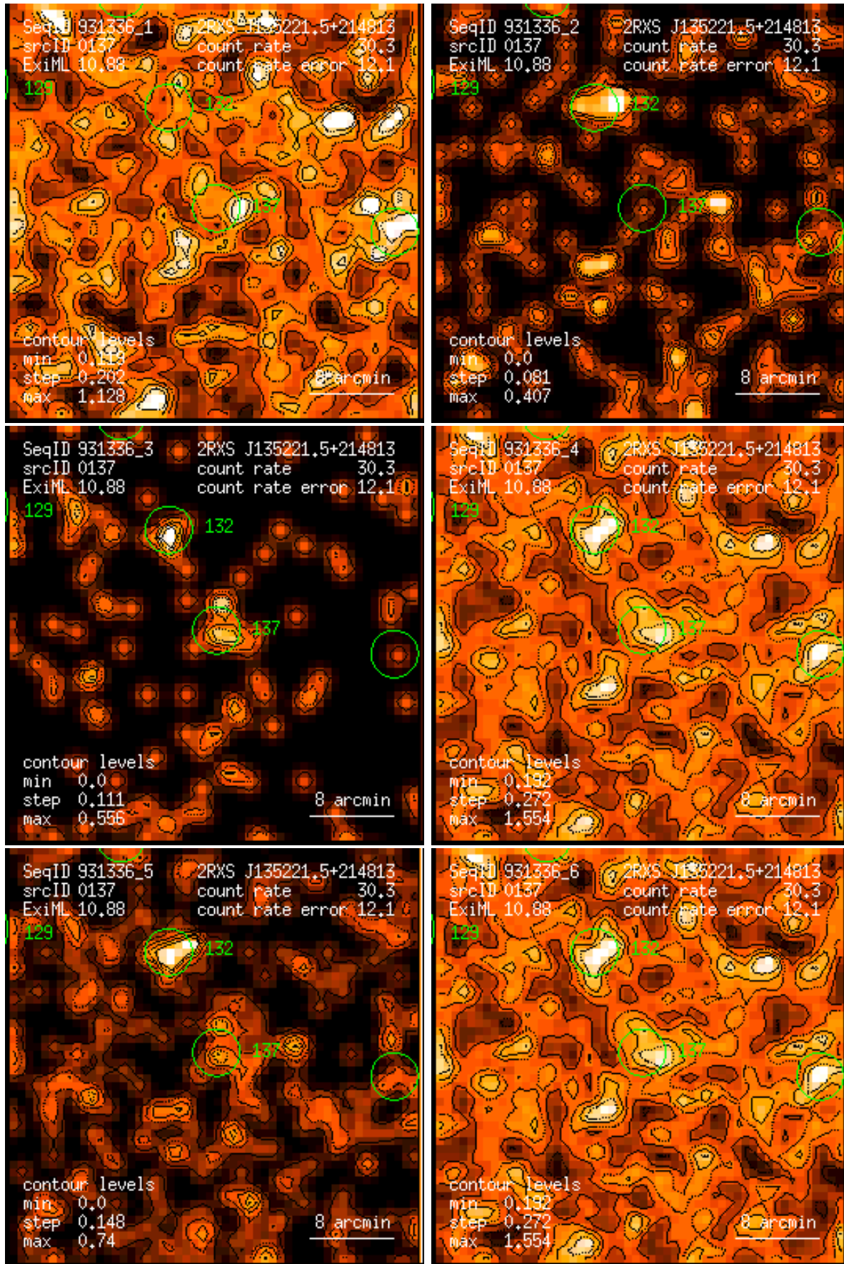
Figure 137: RASS 931336: detection 0137: band rate images, Gaussian filter: (1) PSPC channels 11 – 41, (2) 52 – 90, (3) 91 – 201, (4) 11 – 235, (5) 52 – 201, (6) 11 – 201. Broad band rates in counts/ks. Band rate contour levels in counts/ks/arcmin 2 .
