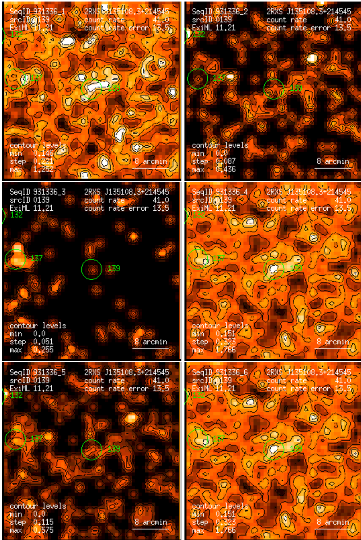
Figure 139: RASS 931336: detection 0139: band rate images, Gaussian filter: (1) PSPC channels 11 – 41, (2) 52 – 90, (3) 91 – 201, (4) 11 – 235, (5) 52 – 201, (6) 11 – 201. Broad band rates in counts/ks. Band rate contour levels in counts/ks/arcmin 2 .
