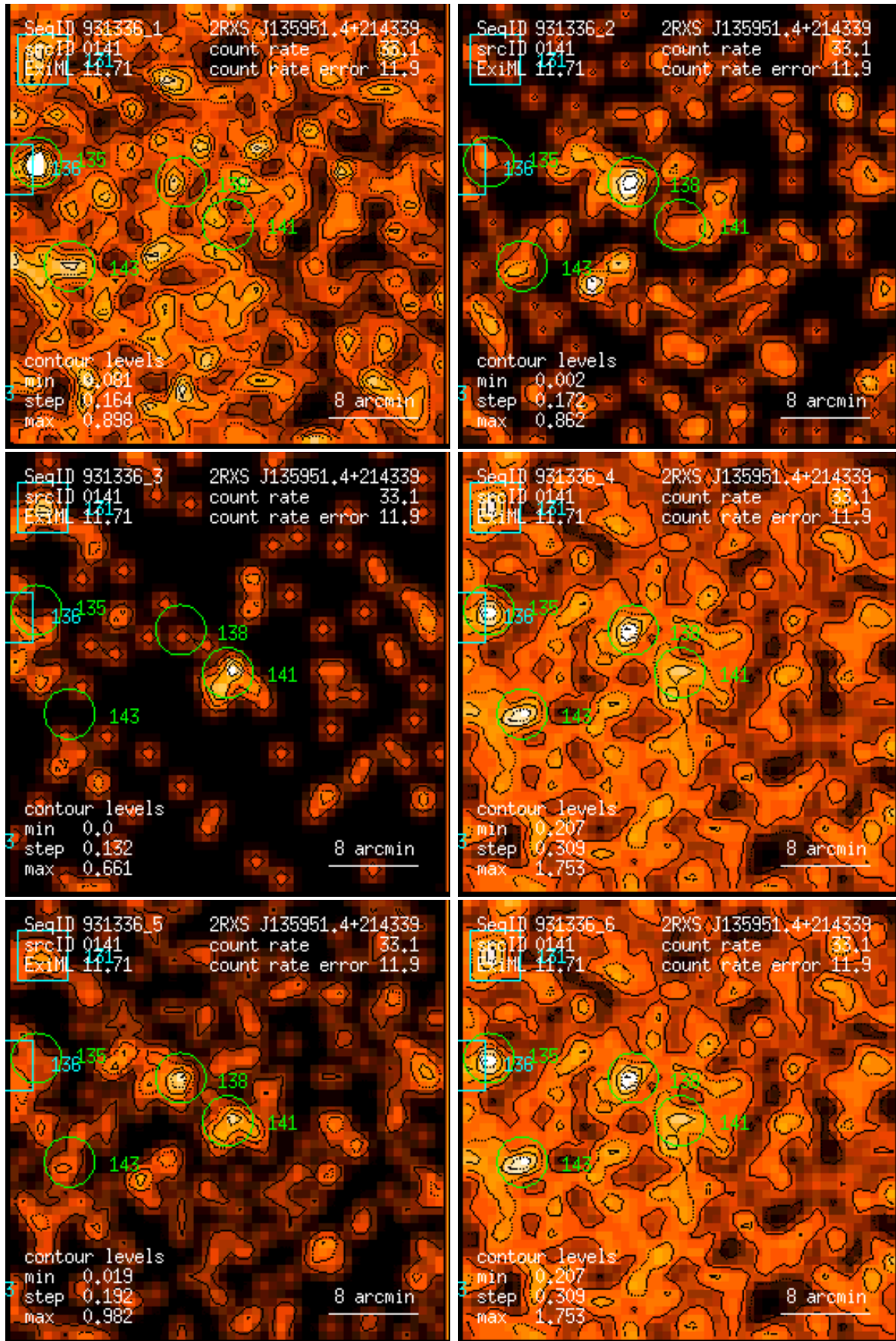
Figure 141: RASS 931336: detection 0141: band rate images, Gaussian filter: (1) PSPC channels 11 – 41, (2) 52 – 90, (3) 91 – 201, (4) 11 – 235, (5) 52 – 201, (6) 11 – 201. Broad band rates in counts/ks. Band rate contour levels in counts/ks/arcmin 2 .
