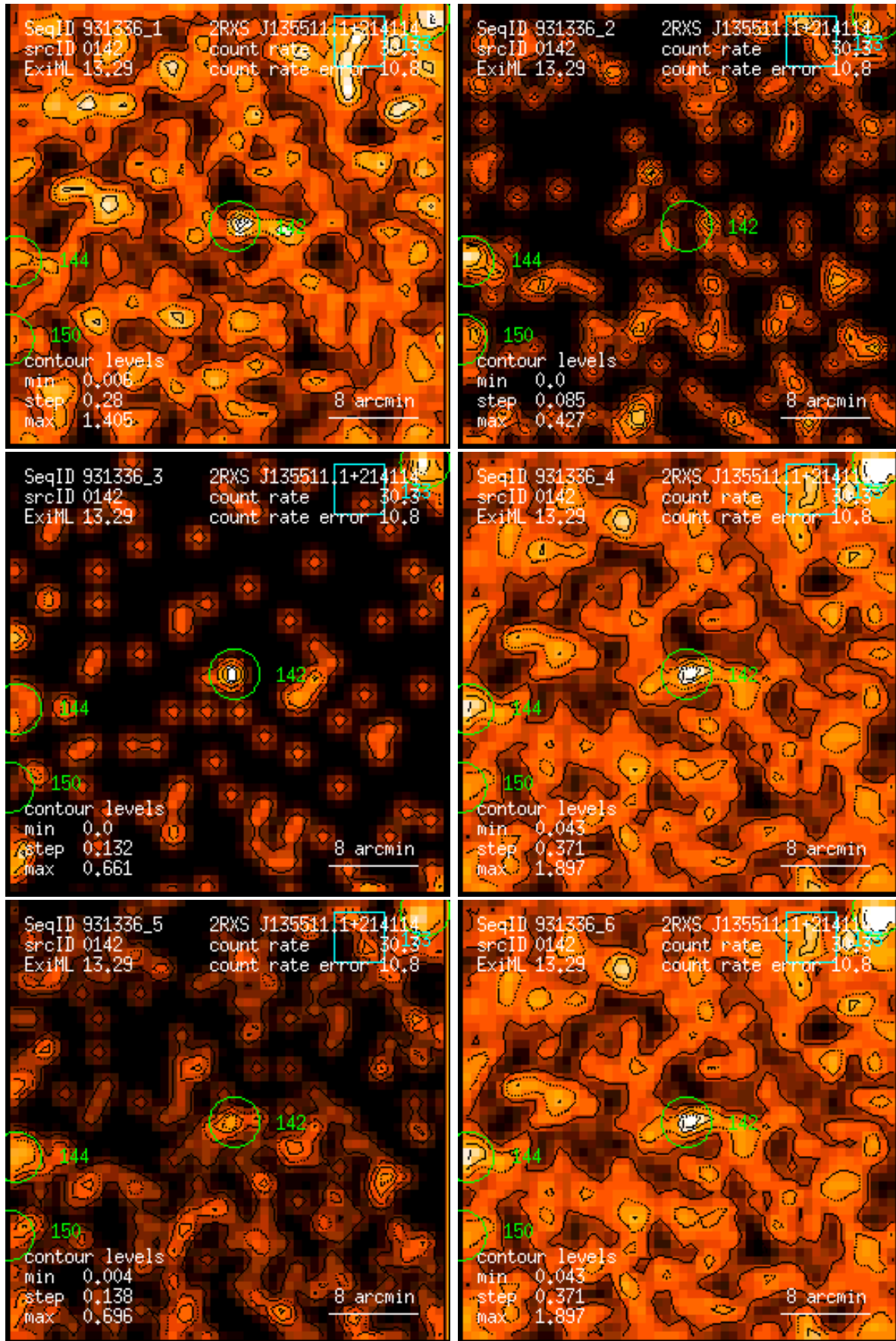
Figure 142: RASS 931336: detection 0142: band rate images, Gaussian filter: (1) PSPC channels 11 – 41, (2) 52 – 90, (3) 91 – 201, (4) 11 – 235, (5) 52 – 201, (6) 11 – 201. Broad band rates in counts/ks. Band rate contour levels in counts/ks/arcmin 2 .
