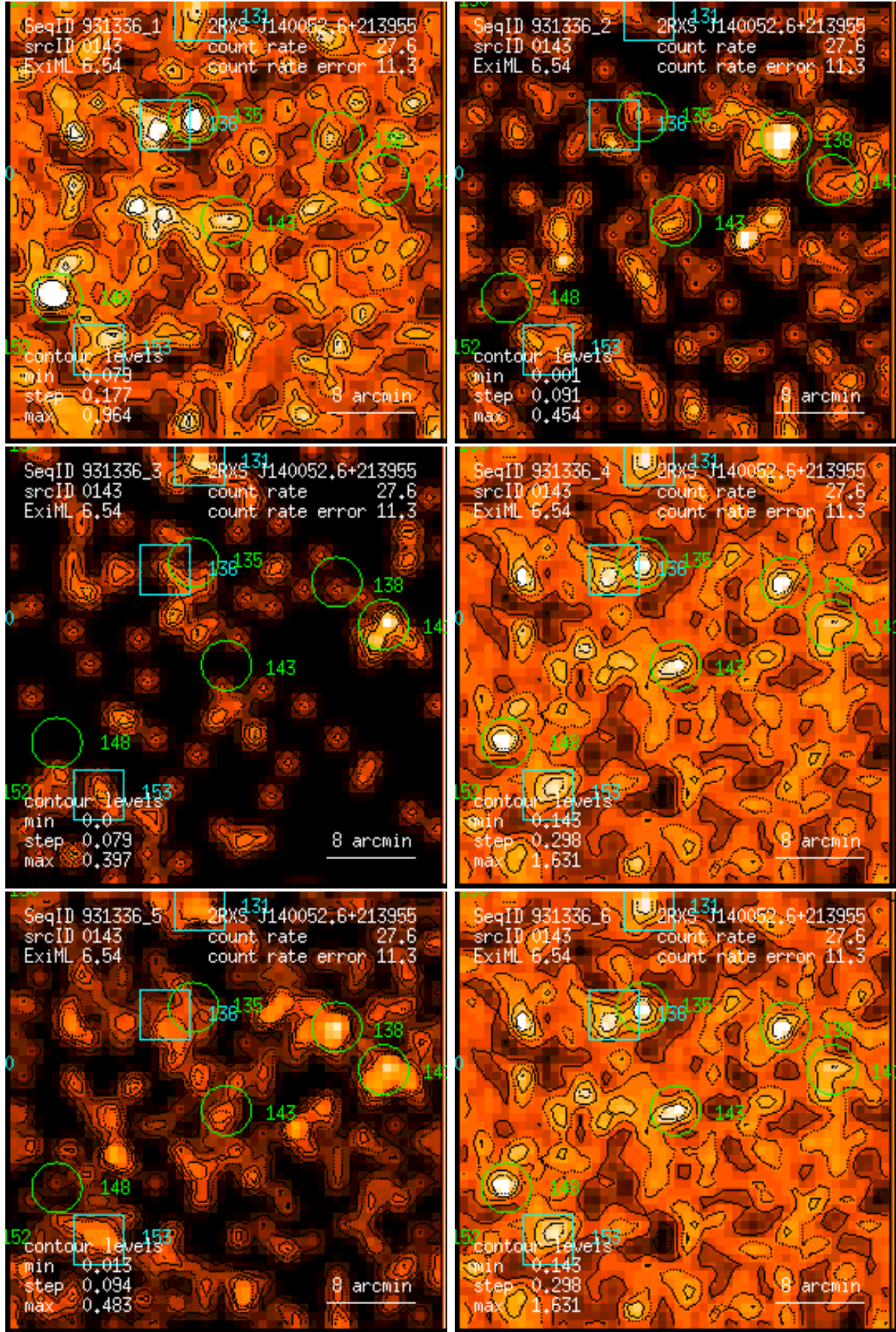
Figure 143: RASS 931336: detection 0143: band rate images, Gaussian filter: (1) PSPC channels 11 – 41, (2) 52 – 90, (3) 91 – 201, (4) 11 – 235, (5) 52 – 201, (6) 11 – 201. Broad band rates in counts/ks. Band rate contour levels in counts/ks/arcmin 2 .
