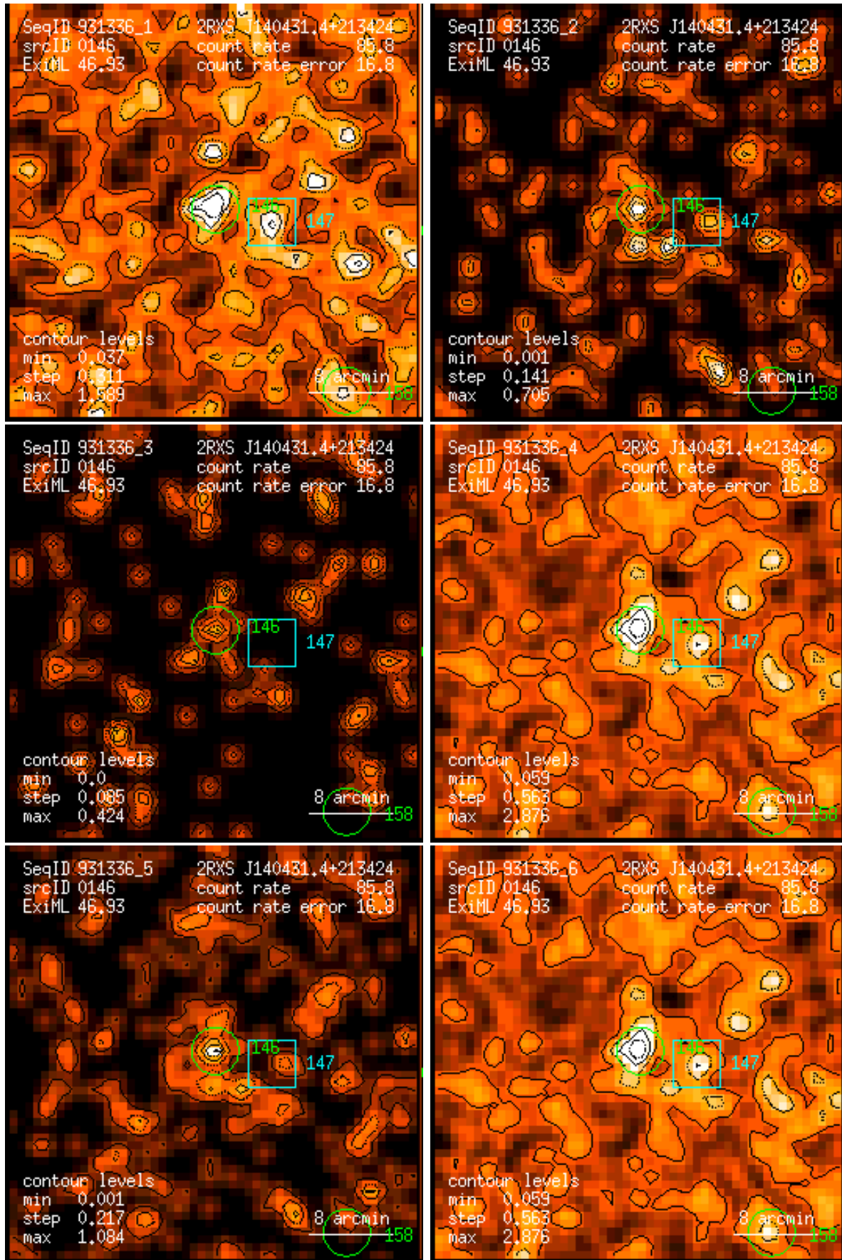
Figure 146: RASS 931336: detection 0146: band rate images, Gaussian filter: (1) PSPC channels 11 – 41, (2) 52 – 90, (3) 91 – 201, (4) 11 – 235, (5) 52 – 201, (6) 11 – 201. Broad band rates in counts/ks. Band rate contour levels in counts/ks/arcmin 2 .
