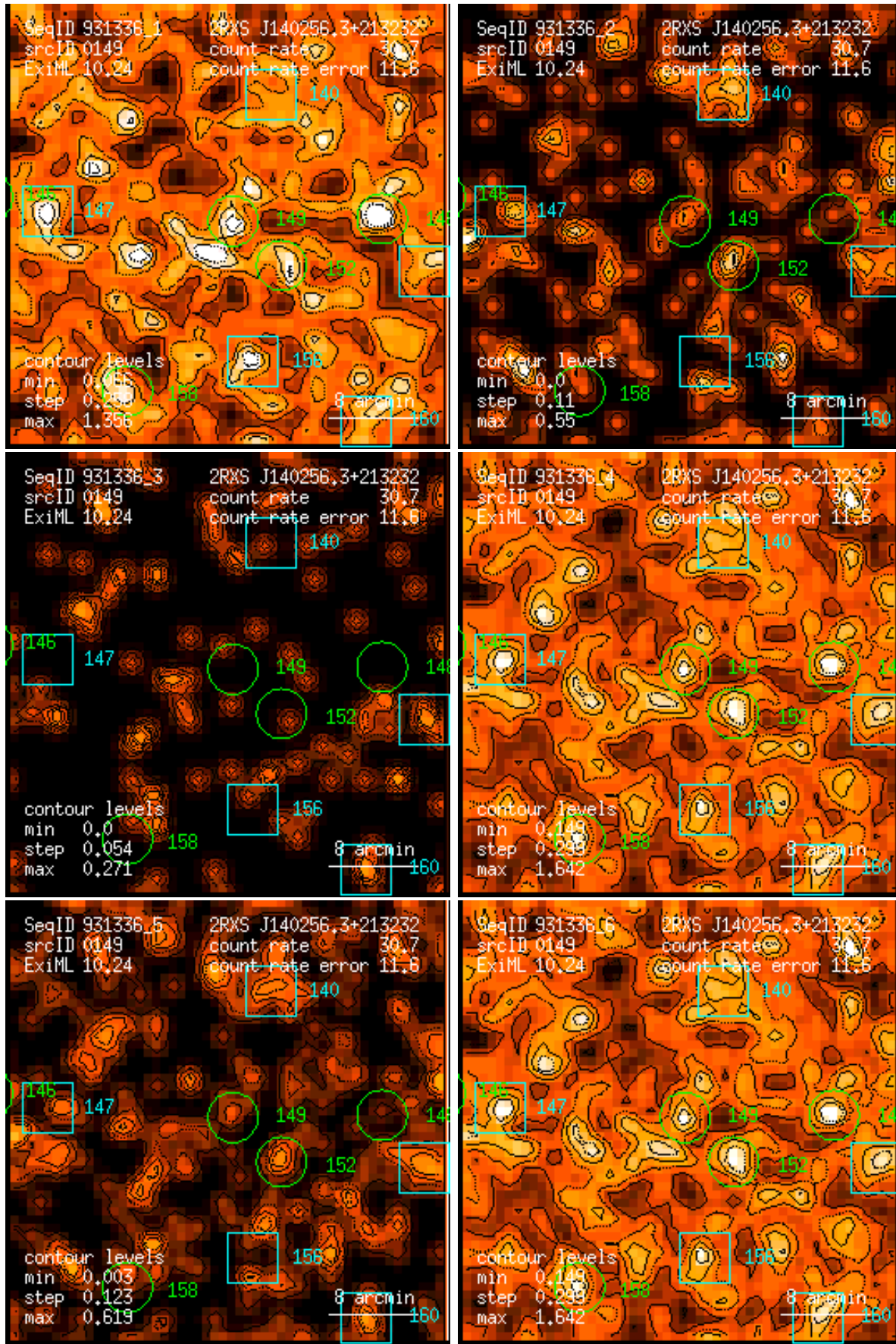
Figure 149: RASS 931336: detection 0149: band rate images, Gaussian filter: (1) PSPC channels 11 – 41, (2) 52 – 90, (3) 91 – 201, (4) 11 – 235, (5) 52 – 201, (6) 11 – 201. Broad band rates in counts/ks. Band rate contour levels in counts/ks/arcmin 2 .
