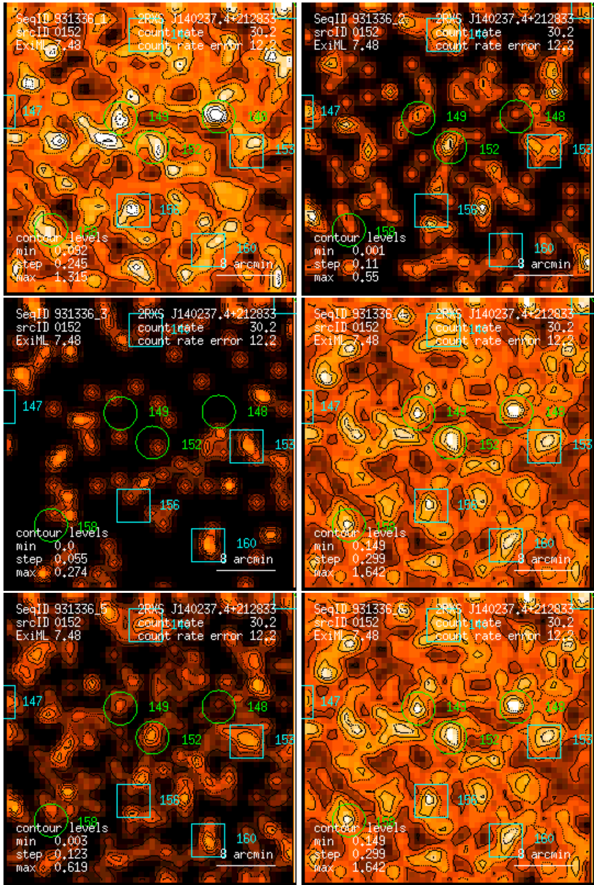
Figure 152: RASS 931336: detection 0152: band rate images, Gaussian filter: (1) PSPC channels 11 – 41, (2) 52 – 90, (3) 91 – 201, (4) 11 – 235, (5) 52 – 201, (6) 11 – 201. Broad band rates in counts/ks. Band rate contour levels in counts/ks/arcmin 2 .
