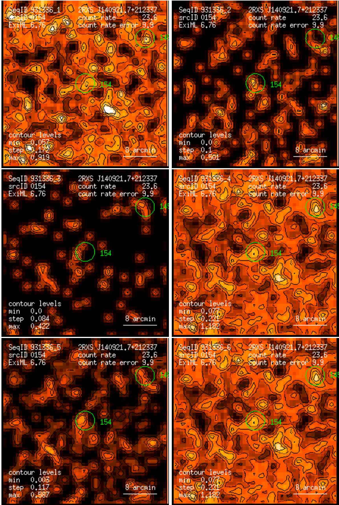
Figure 154: RASS 931336: detection 0154: band rate images, Gaussian filter: (1) PSPC channels 11 – 41, (2) 52 – 90, (3) 91 – 201, (4) 11 – 235, (5) 52 – 201, (6) 11 – 201. Broad band rates in counts/ks. Band rate contour levels in counts/ks/arcmin 2 .
