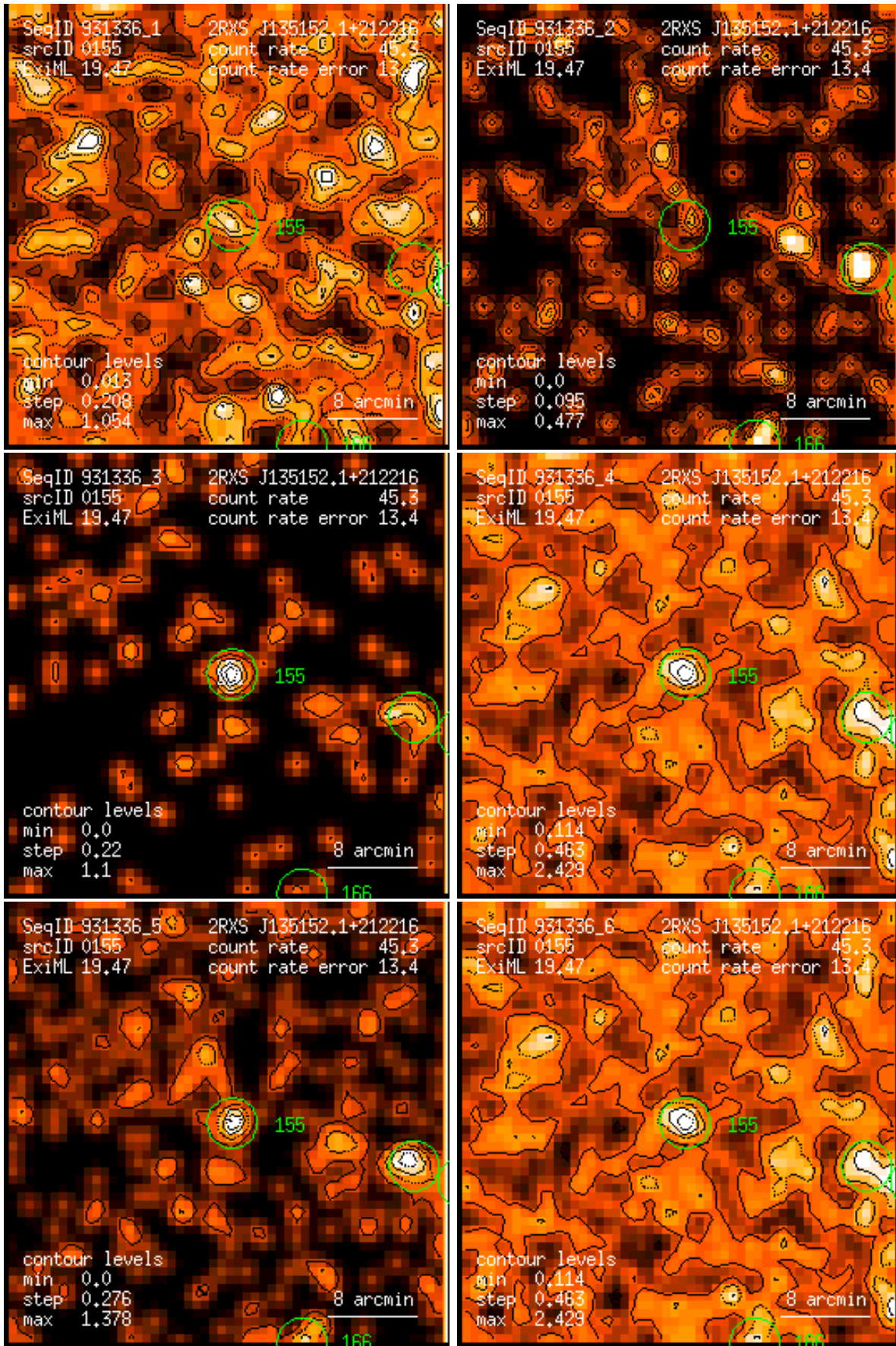
Figure 155: RASS 931336: detection 0155: band rate images, Gaussian filter: (1) PSPC channels 11 – 41, (2) 52 – 90, (3) 91 – 201, (4) 11 – 235, (5) 52 – 201, (6) 11 – 201. Broad band rates in counts/ks. Band rate contour levels in counts/ks/arcmin 2 .
