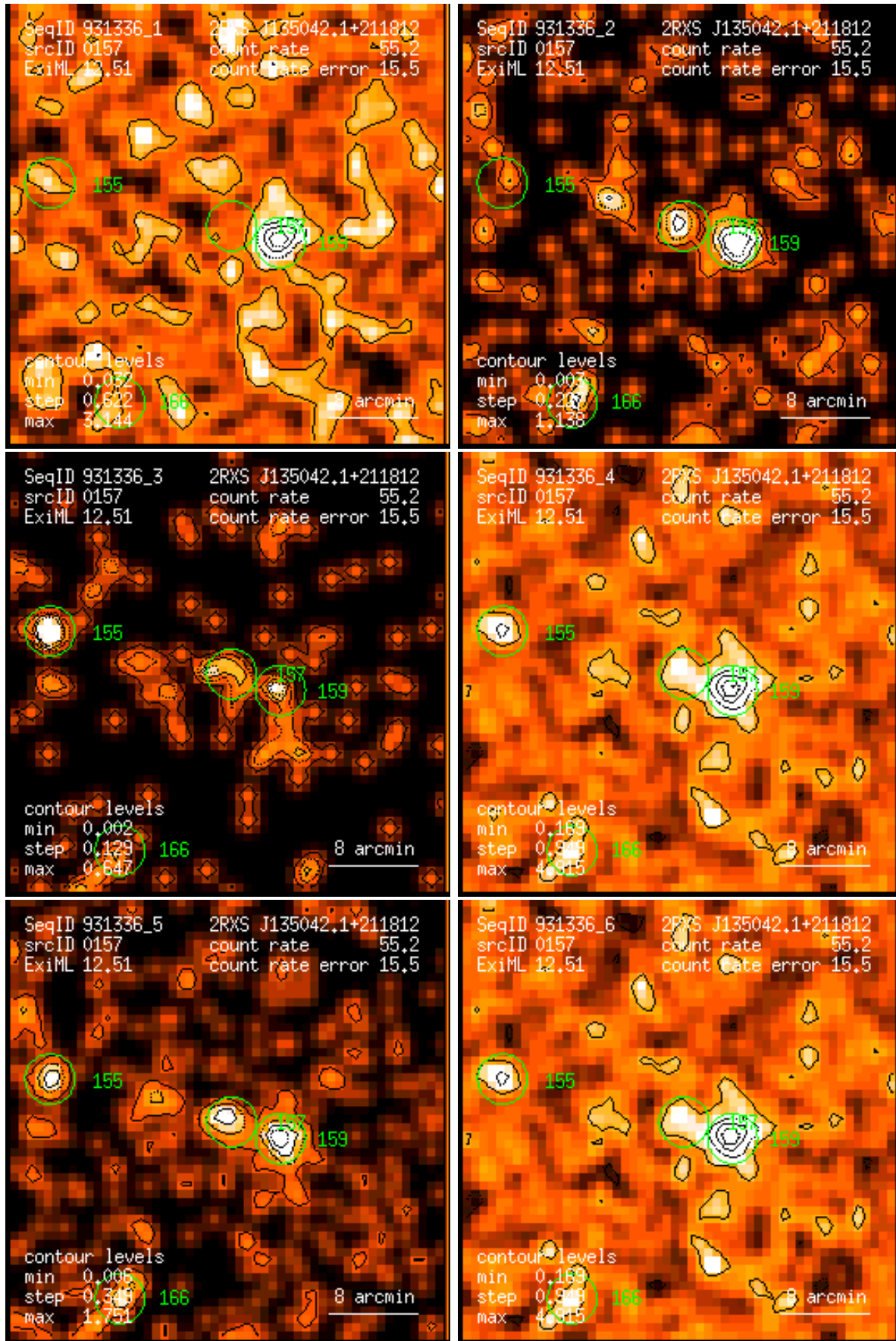
Figure 157: RASS 931336: detection 0157: band rate images, Gaussian filter: (1) PSPC channels 11 – 41, (2) 52 – 90, (3) 91 – 201, (4) 11 – 235, (5) 52 – 201, (6) 11 – 201. Broad band rates in counts/ks. Band rate contour levels in counts/ks/arcmin 2 .
