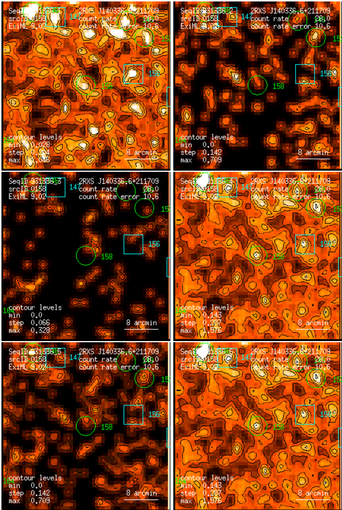
Figure 158: RASS 931336: detection 0158: band rate images, Gaussian filter: (1) PSPC channels 11 – 41, (2) 52 – 90, (3) 91 – 201, (4) 11 – 235, (5) 52 – 201, (6) 11 – 201. Broad band rates in counts/ks. Band rate contour levels in counts/ks/arcmin 2 .
