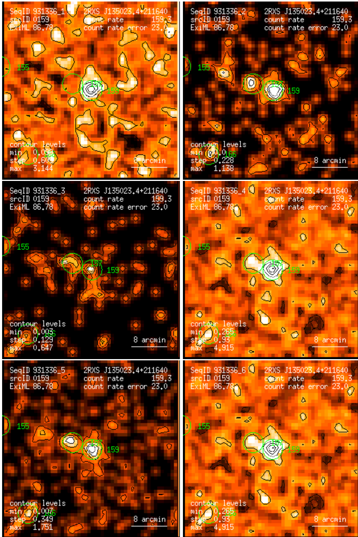
Figure 159: RASS 931336: detection 0159: band rate images, Gaussian filter: (1) PSPC channels 11 – 41, (2) 52 – 90, (3) 91 – 201, (4) 11 – 235, (5) 52 – 201, (6) 11 – 201. Broad band rates in counts/ks. Band rate contour levels in counts/ks/arcmin 2 .
