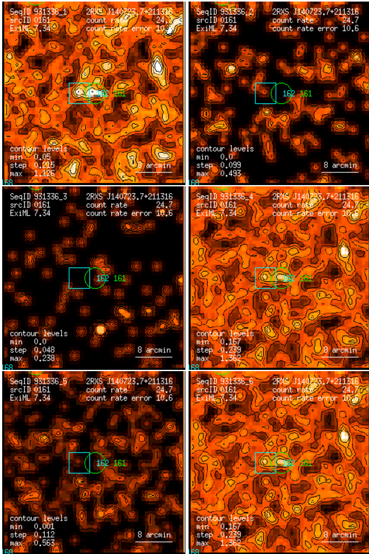
Figure 161: RASS 931336: detection 0161: band rate images, Gaussian filter: (1) PSPC channels 11 – 41, (2) 52 – 90, (3) 91 – 201, (4) 11 – 235, (5) 52 – 201, (6) 11 – 201. Broad band rates in counts/ks. Band rate contour levels in counts/ks/arcmin 2 .
