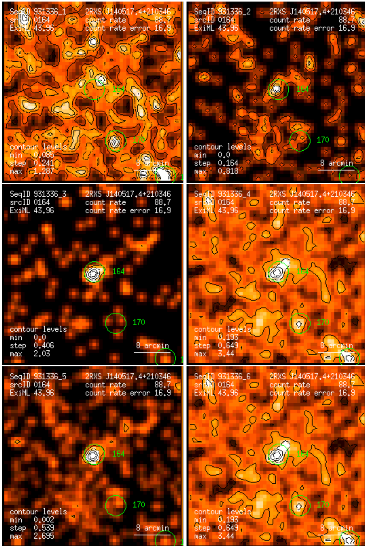
Figure 164: RASS 931336: detection 0164: band rate images, Gaussian filter: (1) PSPC channels 11 – 41, (2) 52 – 90, (3) 91 – 201, (4) 11 – 235, (5) 52 – 201, (6) 11 – 201. Broad band rates in counts/ks. Band rate contour levels in counts/ks/arcmin 2 .
