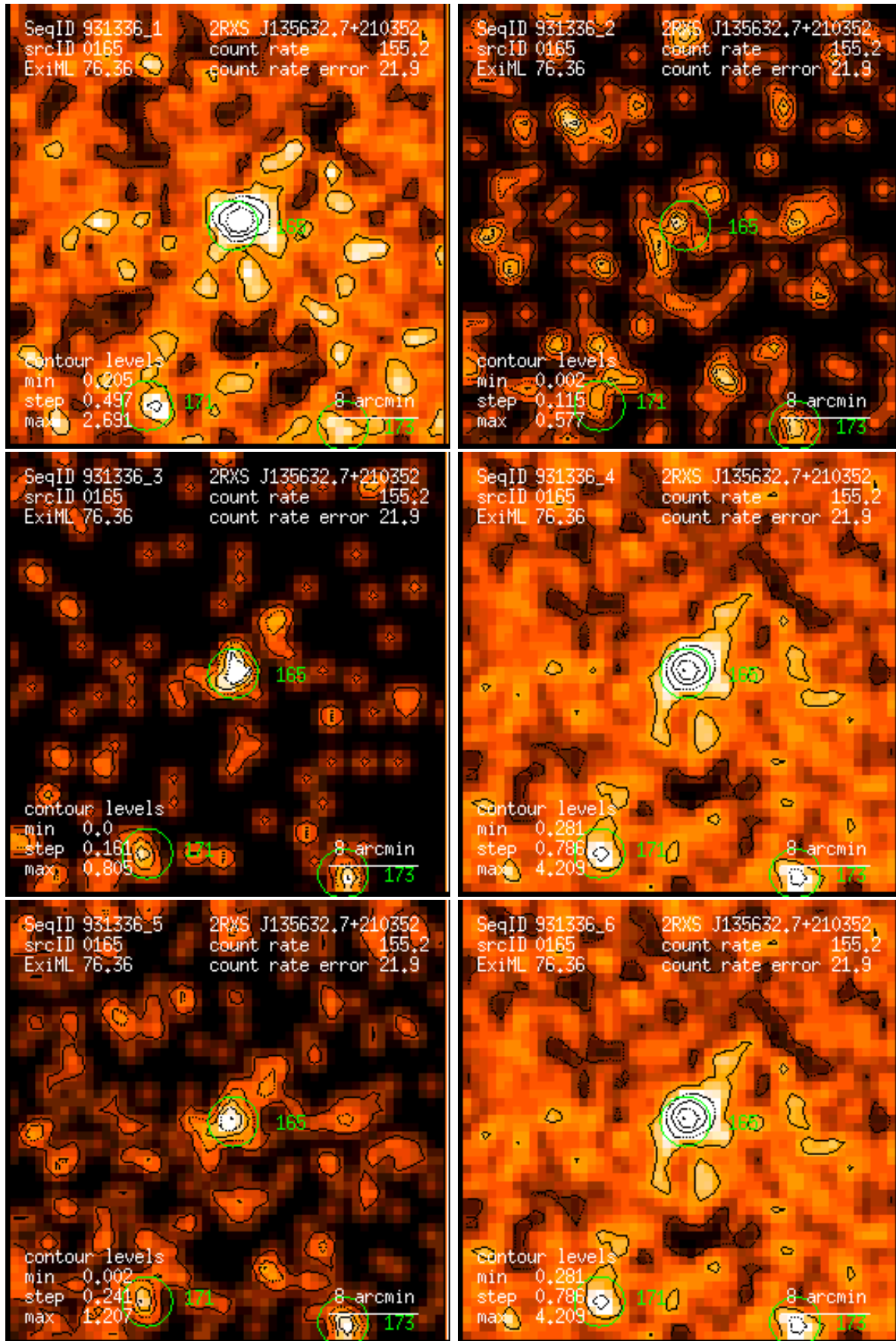
Figure 165: RASS 931336: detection 0165: band rate images, Gaussian filter: (1) PSPC channels 11 – 41, (2) 52 – 90, (3) 91 – 201, (4) 11 – 235, (5) 52 – 201, (6) 11 – 201. Broad band rates in counts/ks. Band rate contour levels in counts/ks/arcmin 2 .
