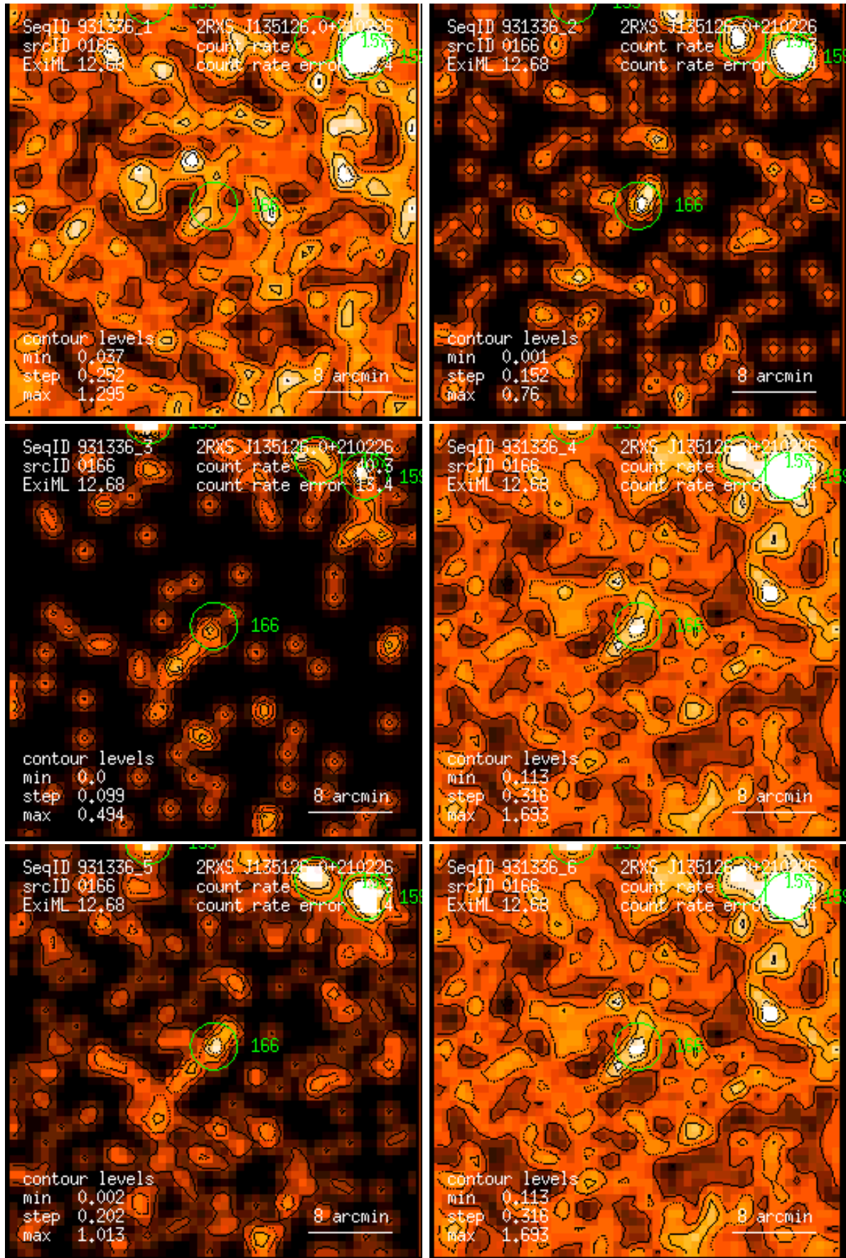
Figure 166: RASS 931336: detection 0166: band rate images, Gaussian filter: (1) PSPC channels 11 – 41, (2) 52 – 90, (3) 91 – 201, (4) 11 – 235, (5) 52 – 201, (6) 11 – 201. Broad band rates in counts/ks. Band rate contour levels in counts/ks/arcmin 2 .
