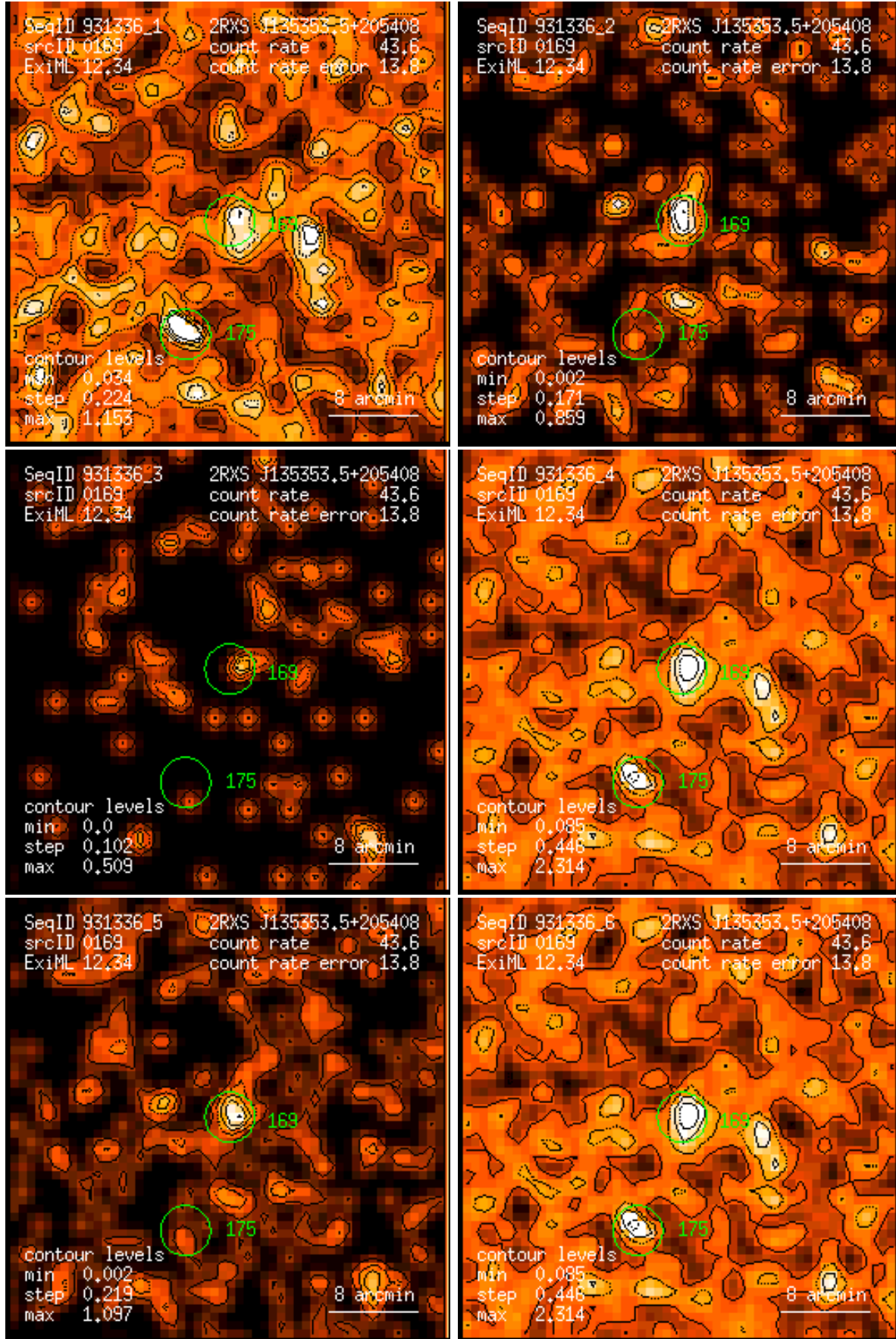
Figure 169: RASS 931336: detection 0169: band rate images, Gaussian filter: (1) PSPC channels 11 – 41, (2) 52 – 90, (3) 91 – 201, (4) 11 – 235, (5) 52 – 201, (6) 11 – 201. Broad band rates in counts/ks. Band rate contour levels in counts/ks/arcmin 2 .
