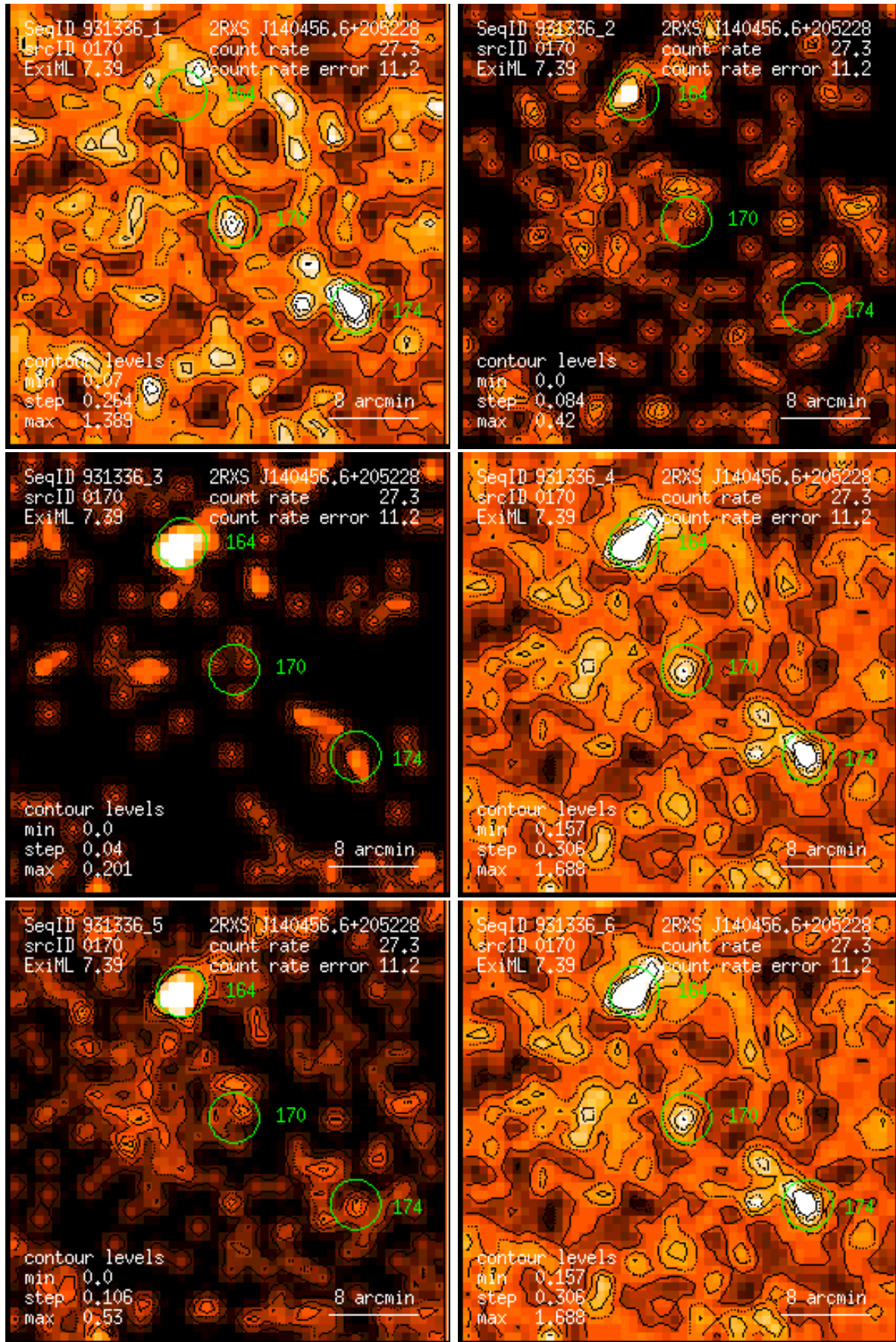
Figure 170: RASS 931336: detection 0170: band rate images, Gaussian filter: (1) PSPC channels 11 – 41, (2) 52 – 90, (3) 91 – 201, (4) 11 – 235, (5) 52 – 201, (6) 11 – 201. Broad band rates in counts/ks. Band rate contour levels in counts/ks/arcmin 2 .
