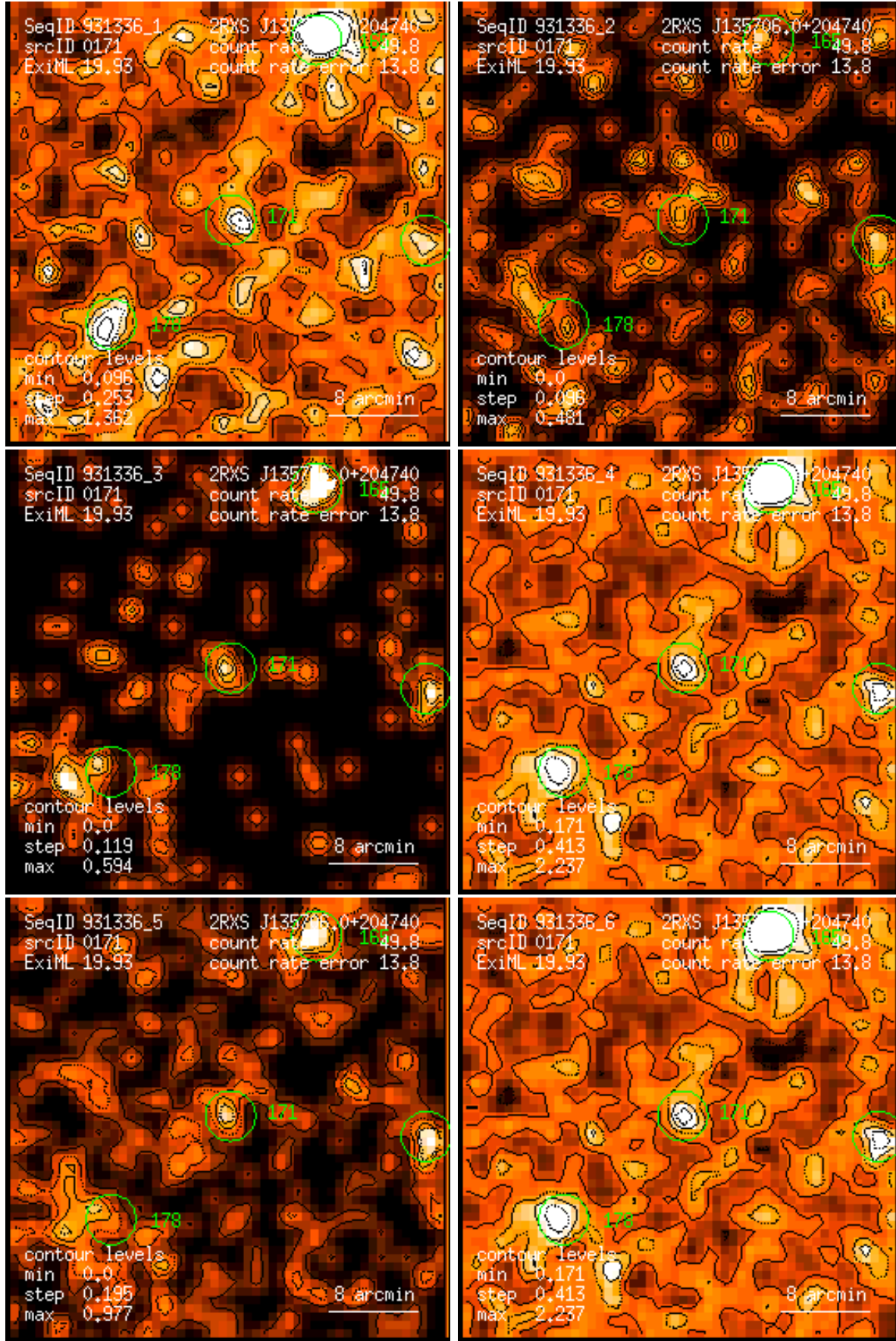
Figure 171: RASS 931336: detection 0171: band rate images, Gaussian filter: (1) PSPC channels 11 – 41, (2) 52 – 90, (3) 91 – 201, (4) 11 – 235, (5) 52 – 201, (6) 11 – 201. Broad band rates in counts/ks. Band rate contour levels in counts/ks/arcmin 2 .
