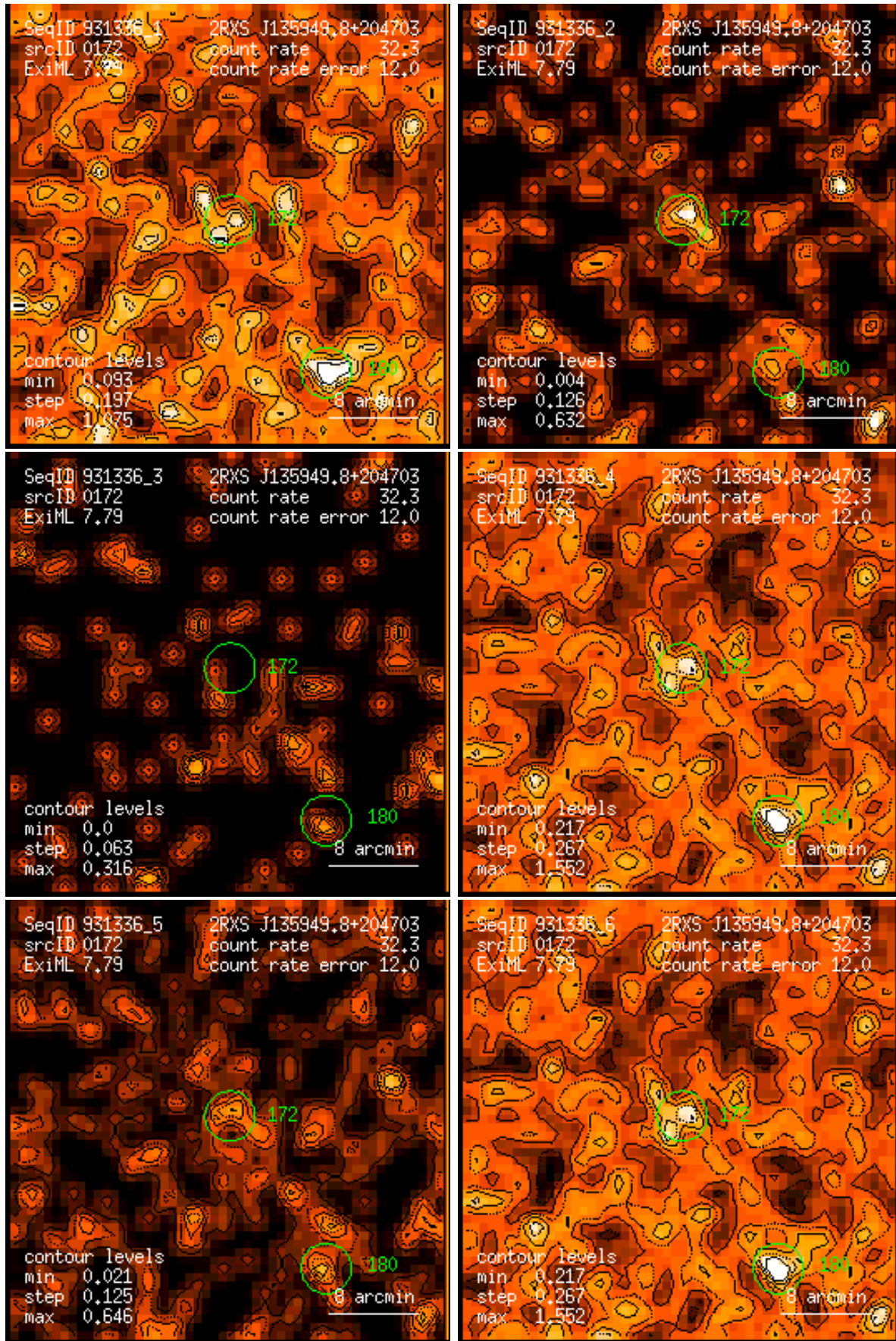
Figure 172: RASS 931336: detection 0172: band rate images, Gaussian filter: (1) PSPC channels 11 – 41, (2) 52 – 90, (3) 91 – 201, (4) 11 – 235, (5) 52 – 201, (6) 11 – 201. Broad band rates in counts/ks. Band rate contour levels in counts/ks/arcmin 2 .
