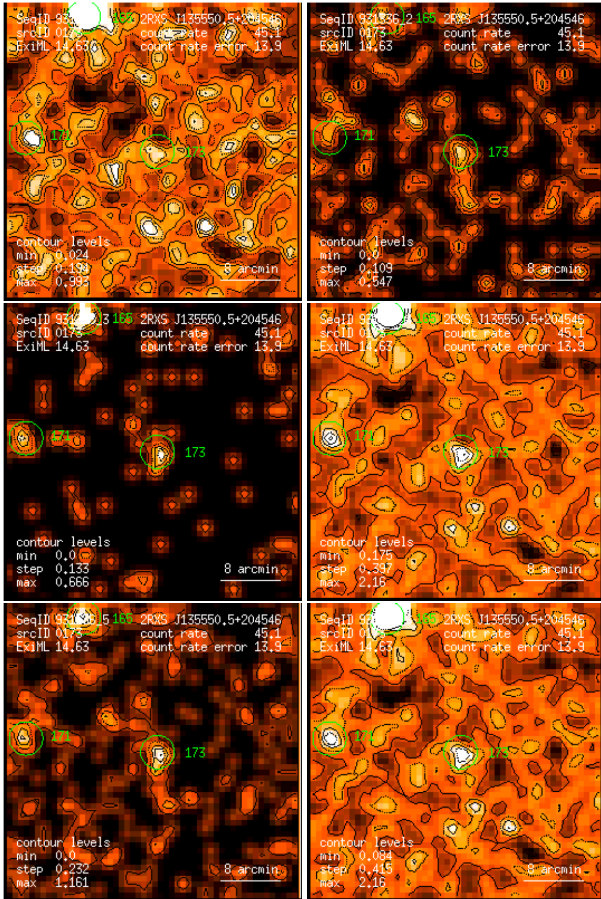
Figure 173: RASS 931336: detection 0173: band rate images, Gaussian filter: (1) PSPC channels 11 – 41, (2) 52 – 90, (3) 91 – 201, (4) 11 – 235, (5) 52 – 201, (6) 11 – 201. Broad band rates in counts/ks. Band rate contour levels in counts/ks/arcmin 2 .
